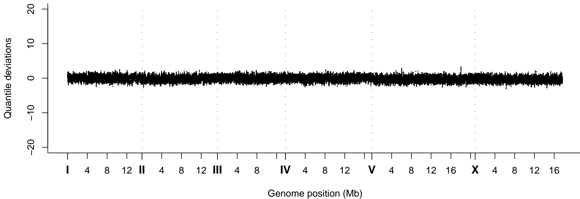
Quantile Deviations, Strain VC30094
