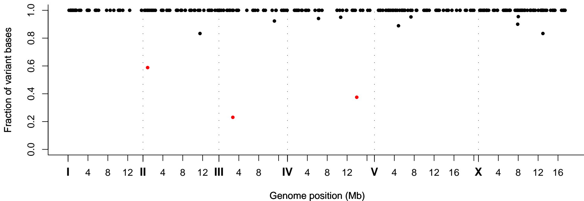
Fraction of Variant Bases at Position, Strain VC30094
