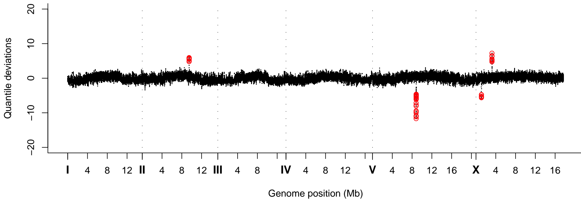
Quantile Deviations, Strain VC30096
