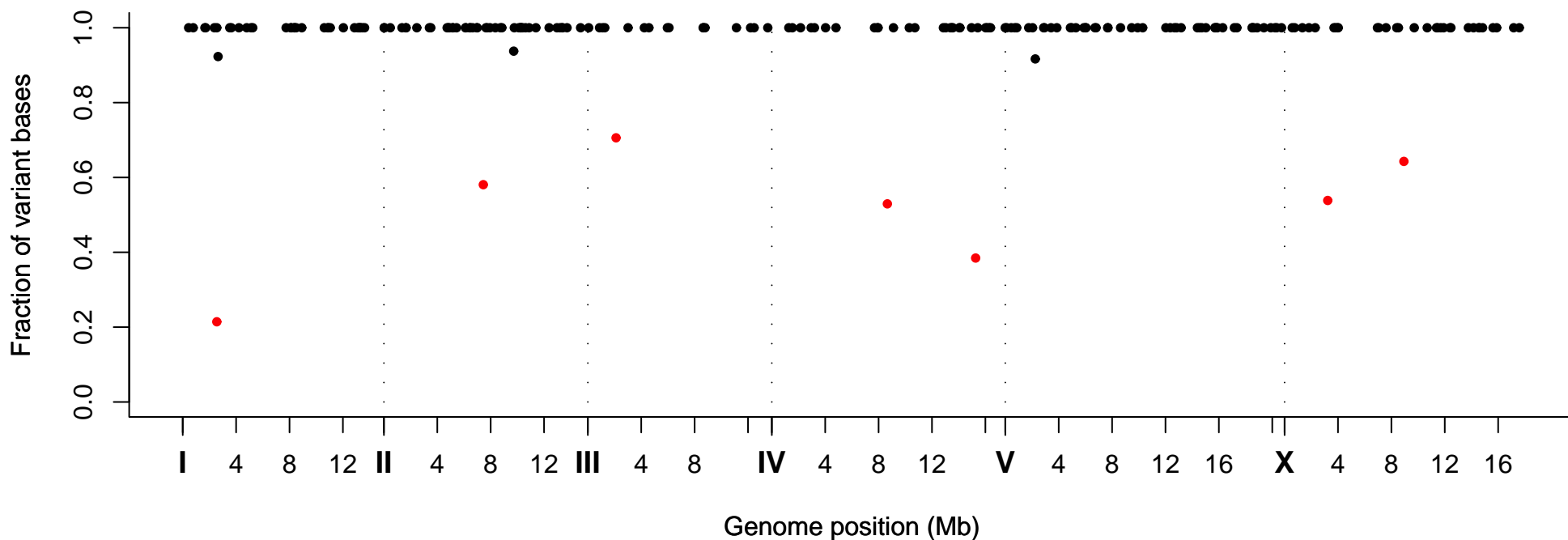
Fraction of Variant Bases at Position, Strain VC30096
