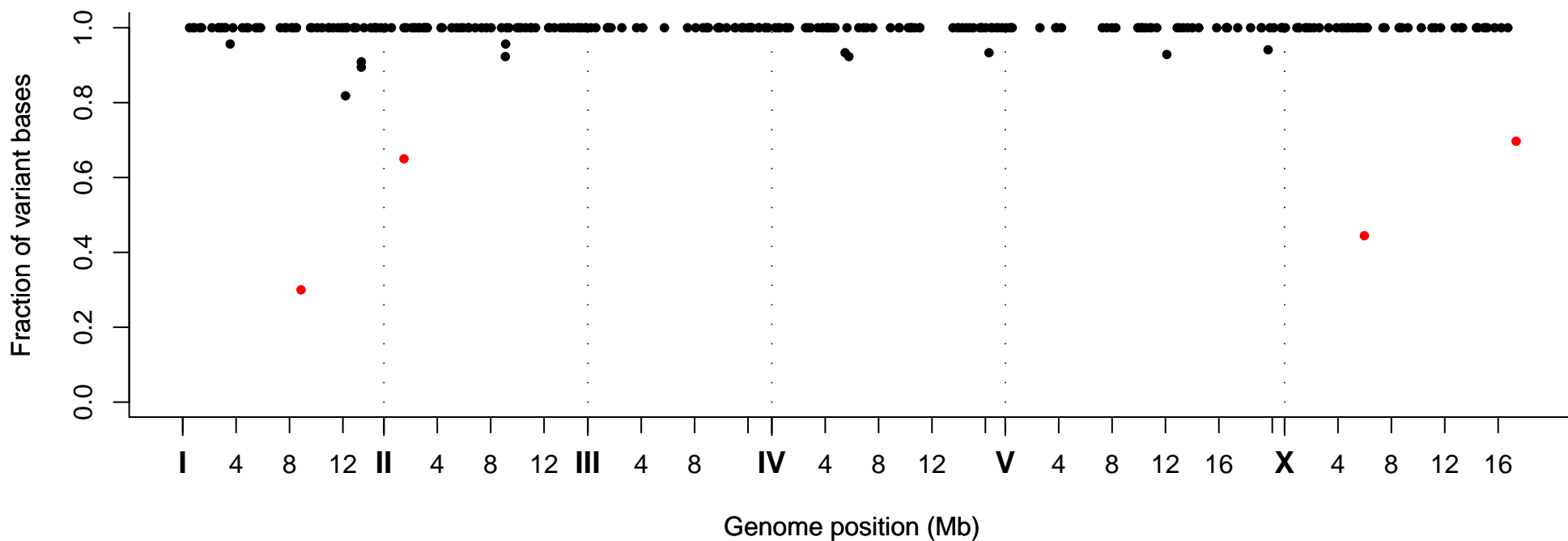
Fraction of Variant Bases at Position, Strain VC30106
