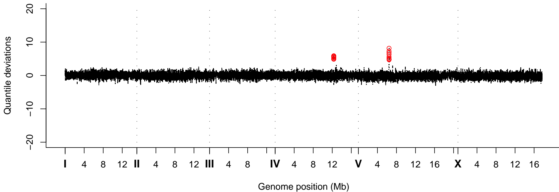
Quantile Deviations, Strain VC30112
