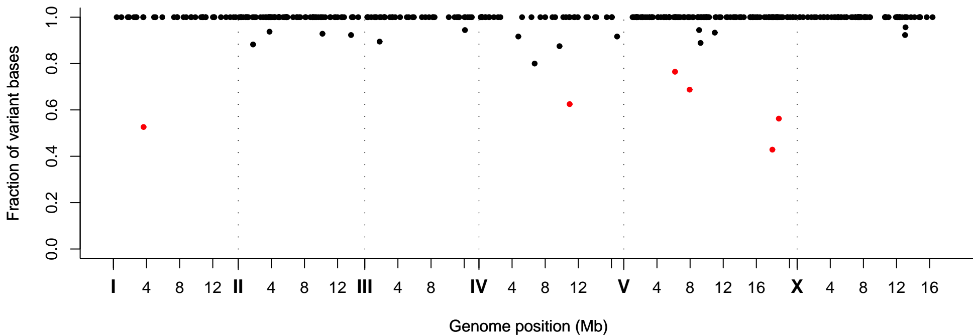
Fraction of Variant Bases at Position, Strain VC30112
