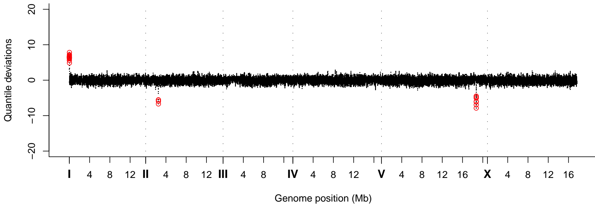
Quantile Deviations, Strain VC30114
