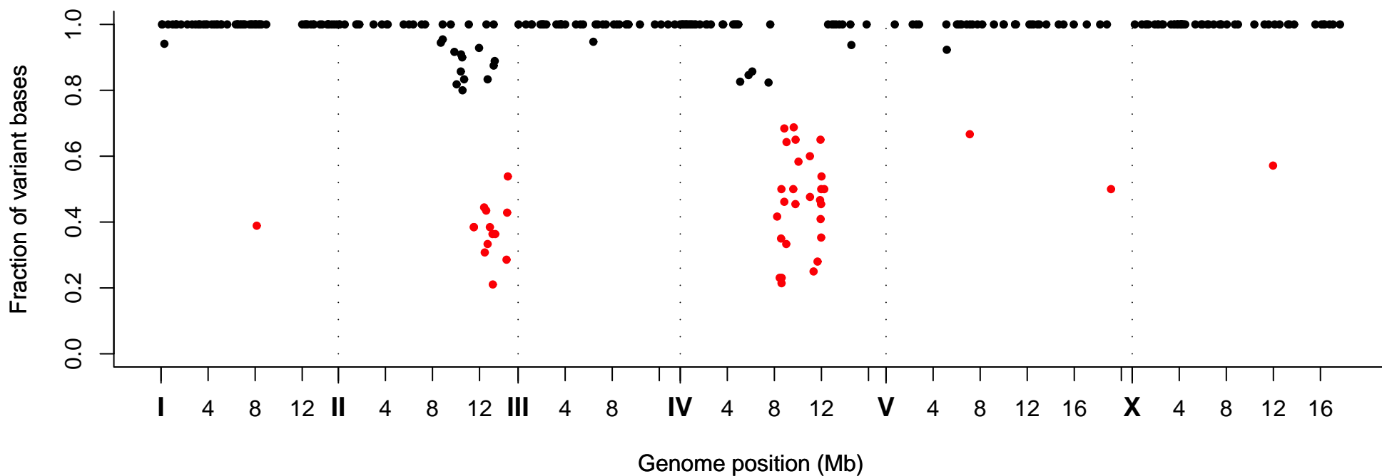
Fraction of Variant Bases at Position, Strain VC30114
