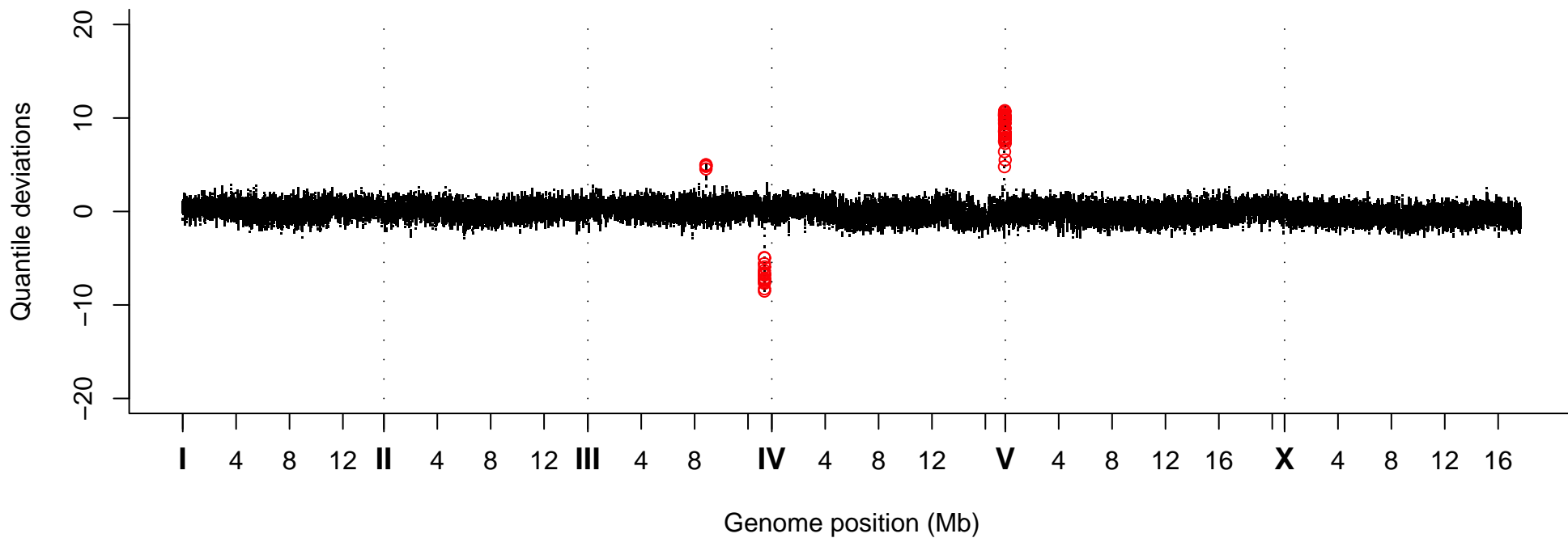
Quantile Deviations, Strain VC30121
