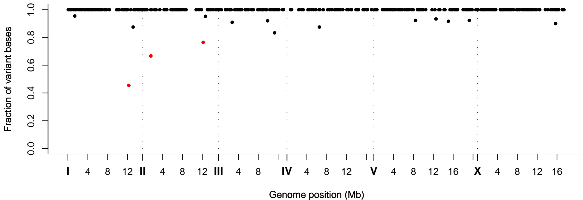
Fraction of Variant Bases at Position, Strain VC30121
