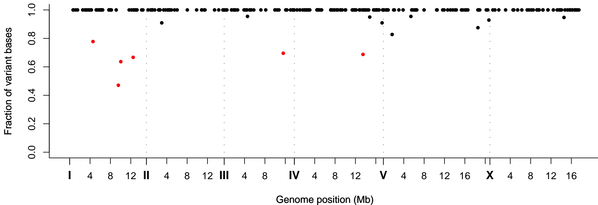
Fraction of Variant Bases at Position, Strain VC30127
