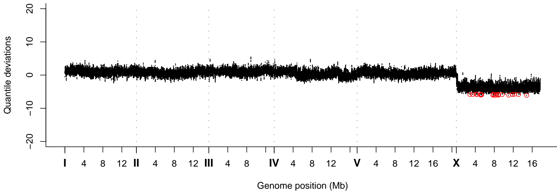
Quantile Deviations, Strain VC30127
