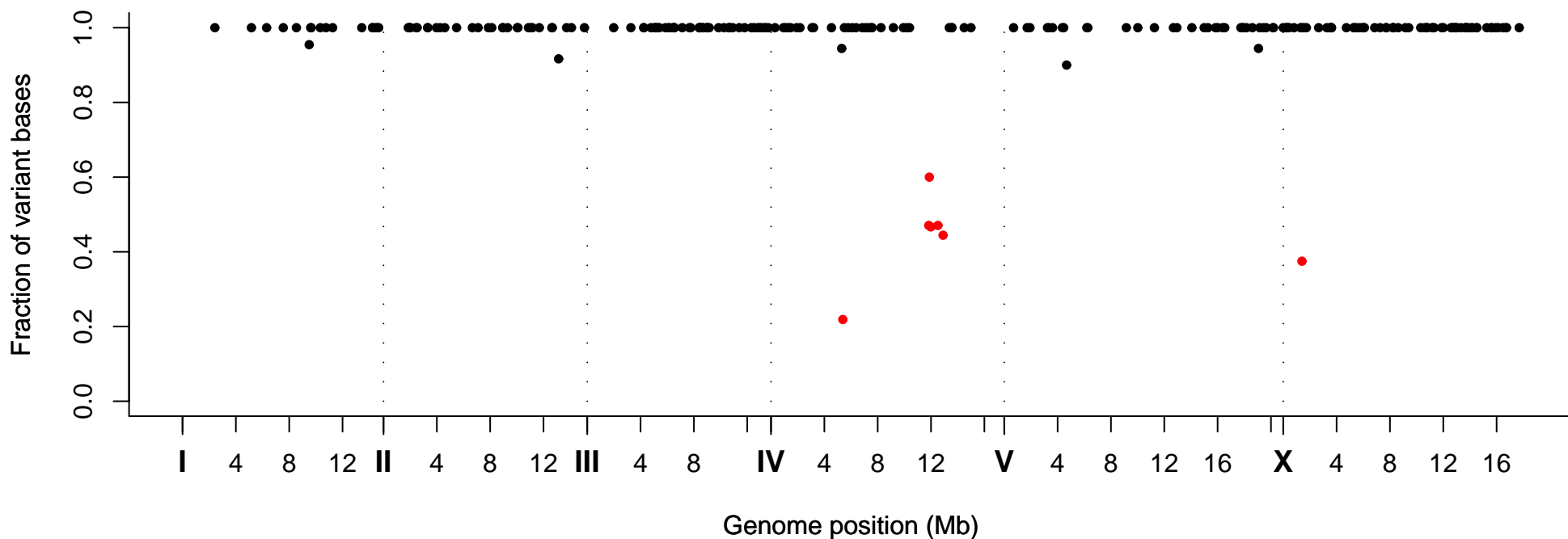
Fraction of Variant Bases at Position, Strain VC30156
