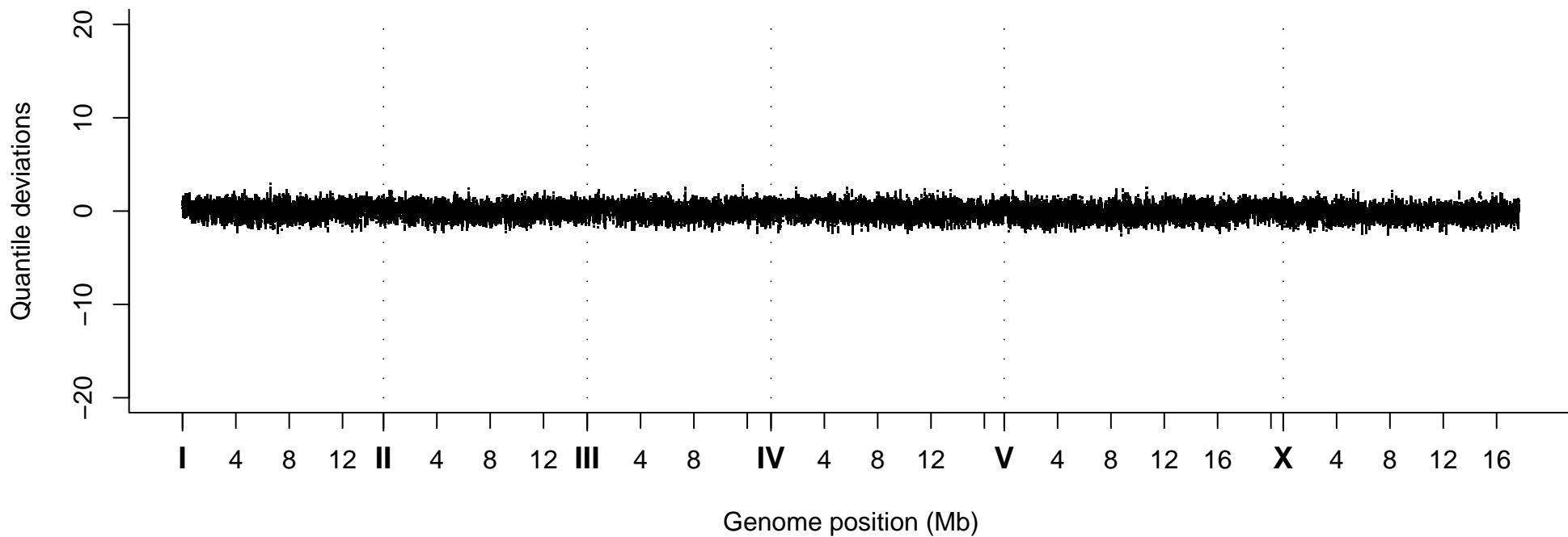
Quantile Deviations, Strain VC30157
