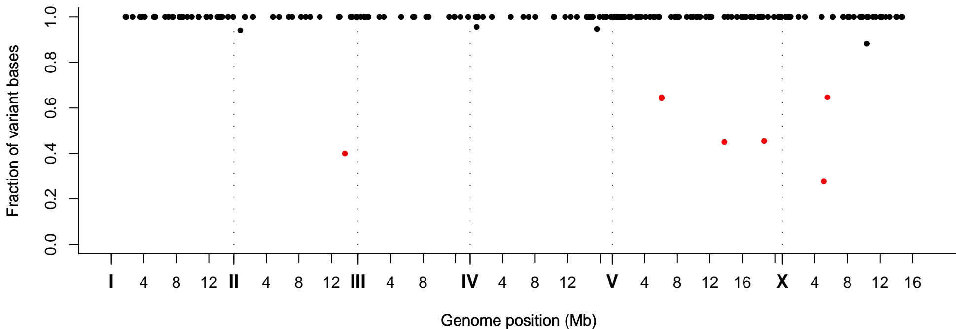
Fraction of Variant Bases at Position, Strain VC30157
