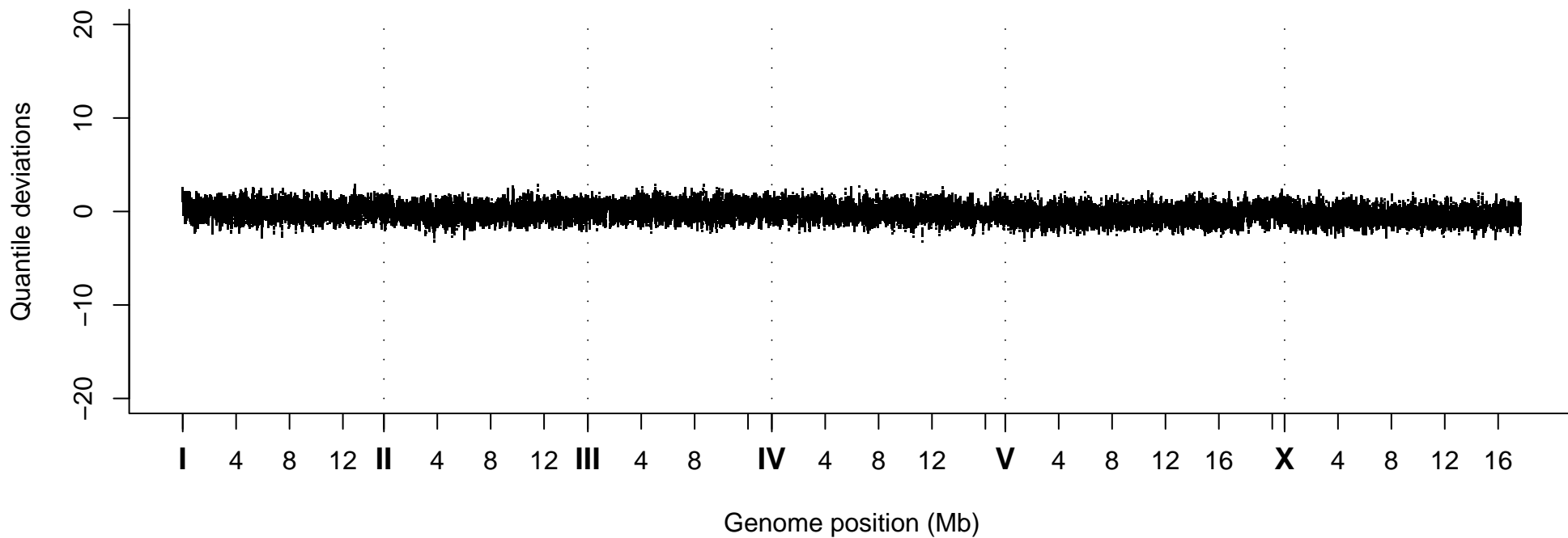
Quantile Deviations, Strain VC30158
