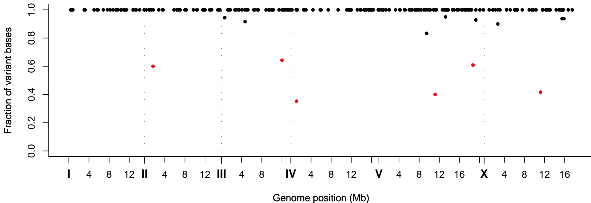
Fraction of Variant Bases at Position, Strain VC30158
