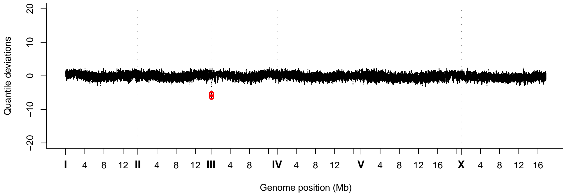
Quantile Deviations, Strain VC30159
