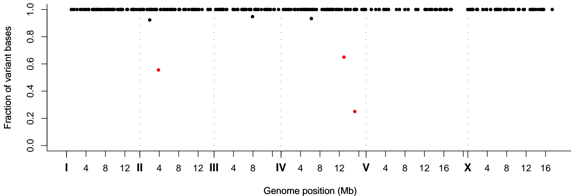
Fraction of Variant Bases at Position, Strain VC30159
