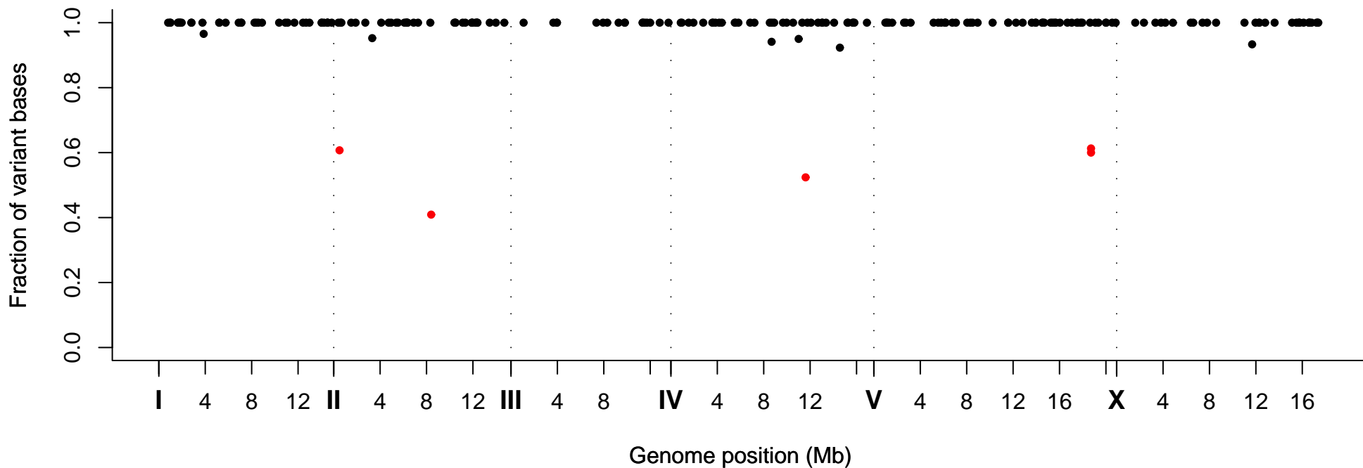
Fraction of Variant Bases at Position, Strain VC30163
