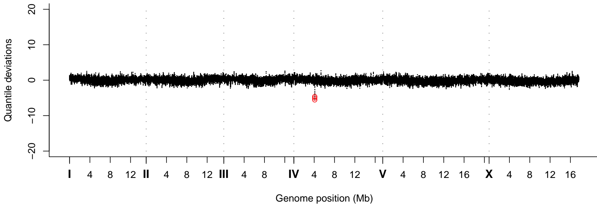
Quantile Deviations, Strain VC30163
