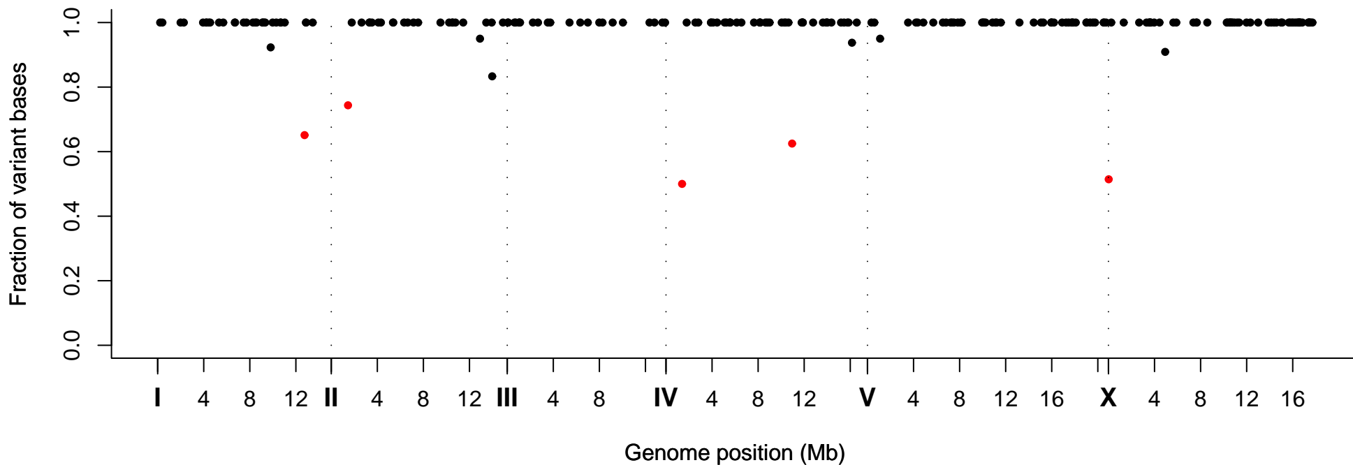
Fraction of Variant Bases at Position, Strain VC30170
