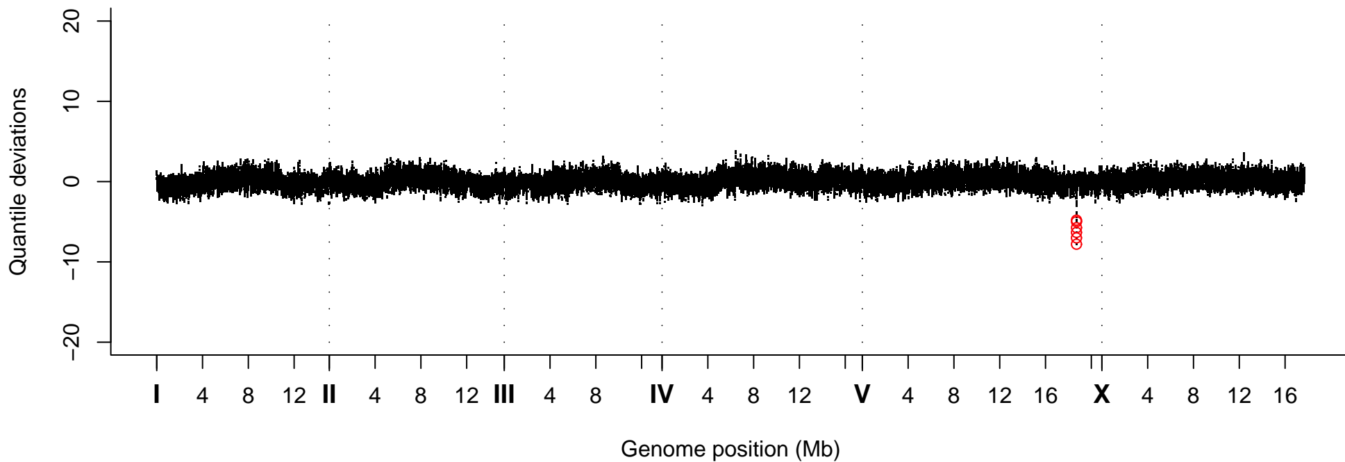
Quantile Deviations, Strain VC30170
