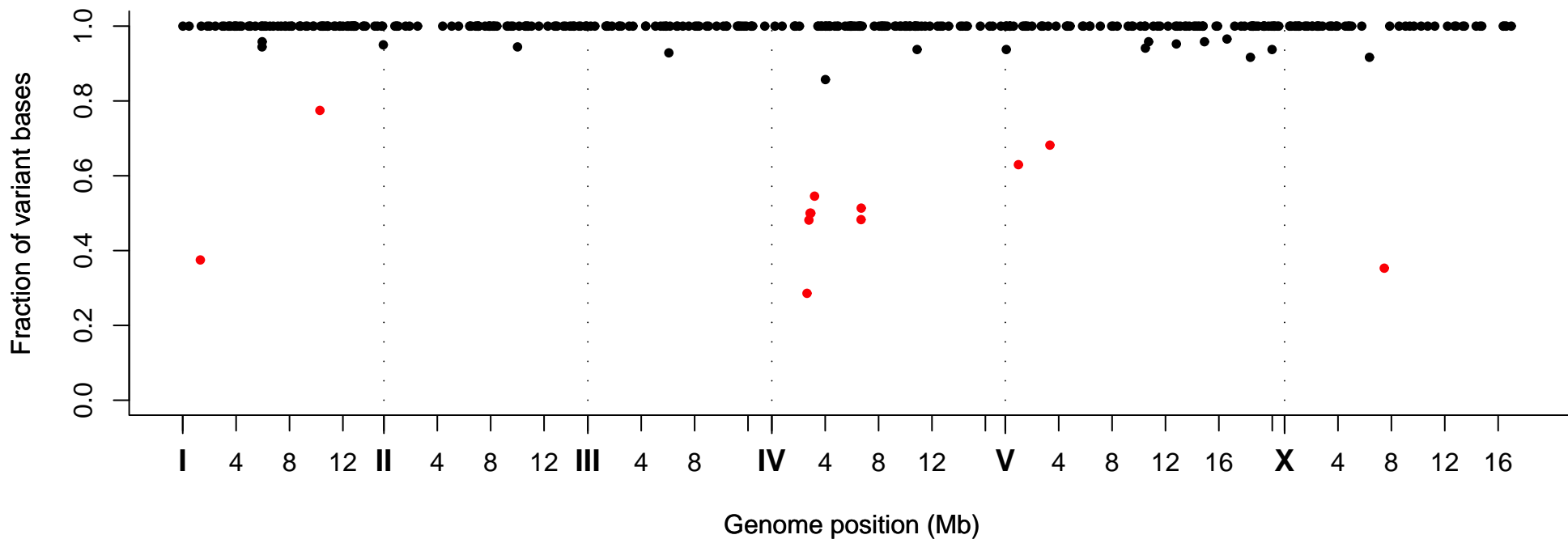
Fraction of Variant Bases at Position, Strain VC30171
