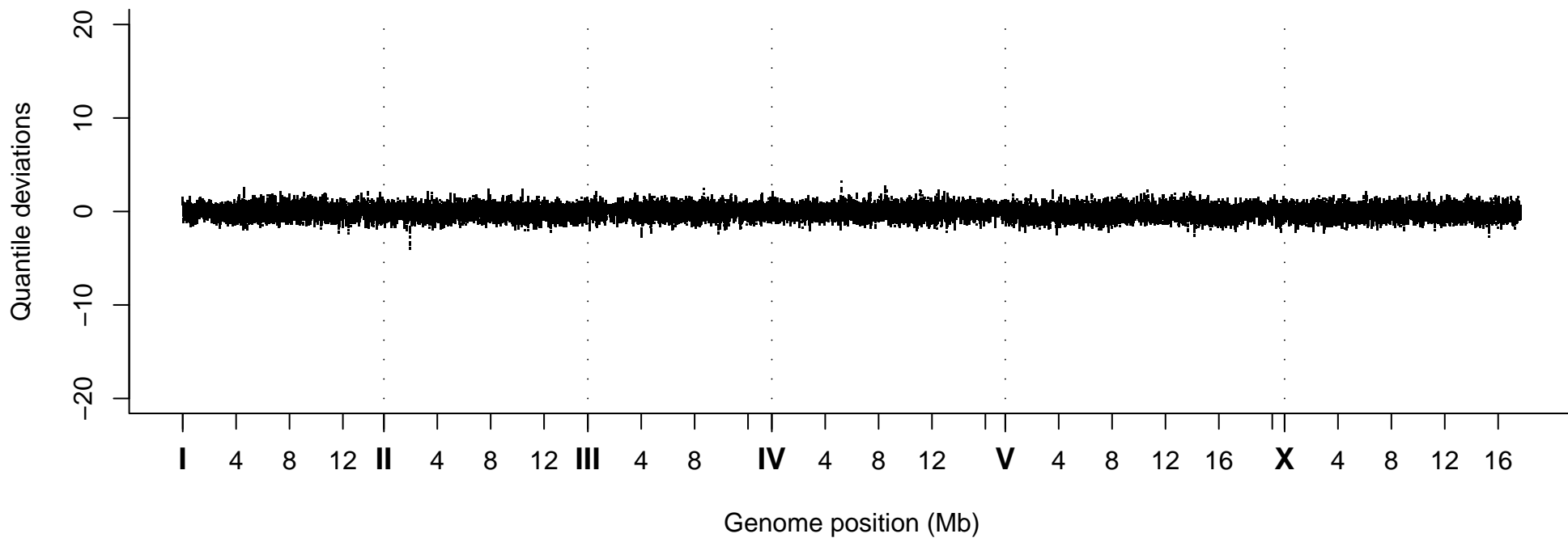
Quantile Deviations, Strain VC30171
