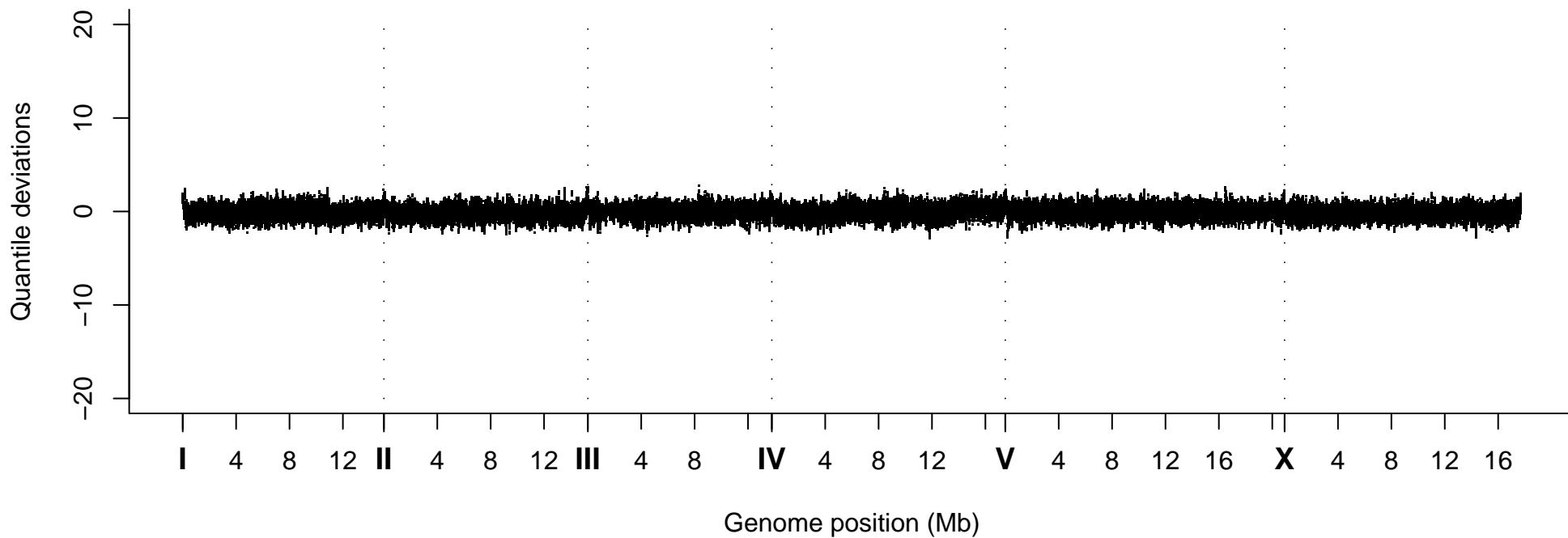
Quantile Deviations, Strain VC30182
