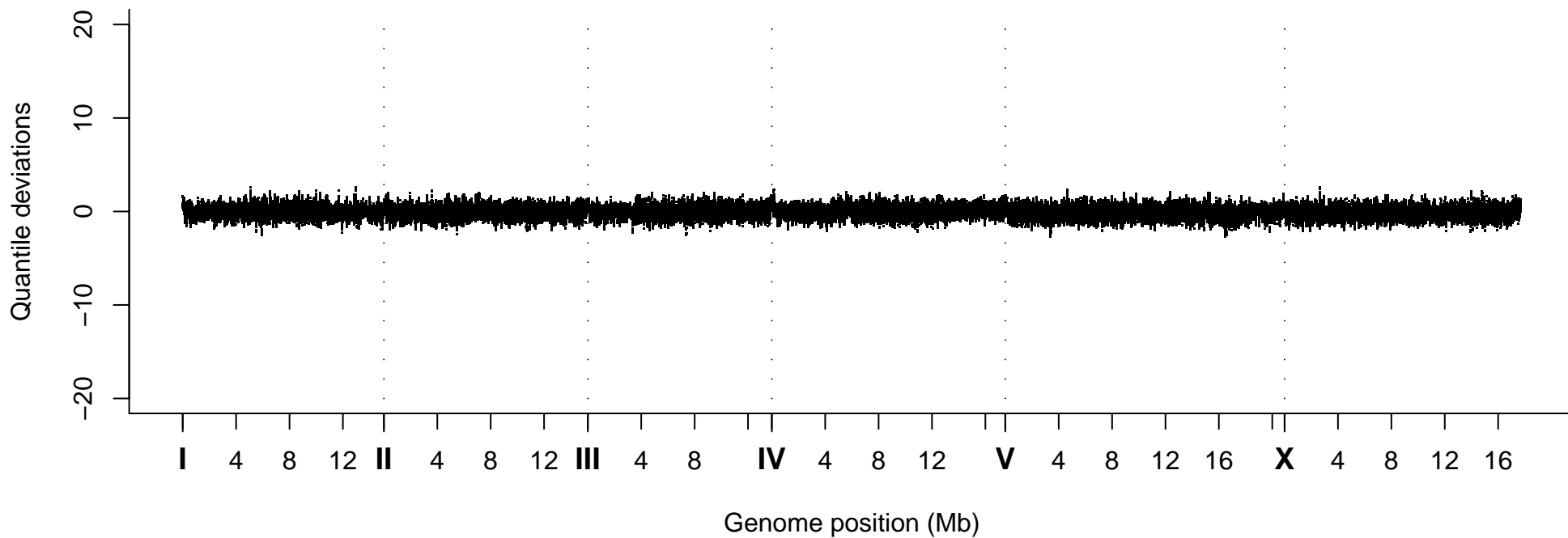
Quantile Deviations, Strain VC30184
