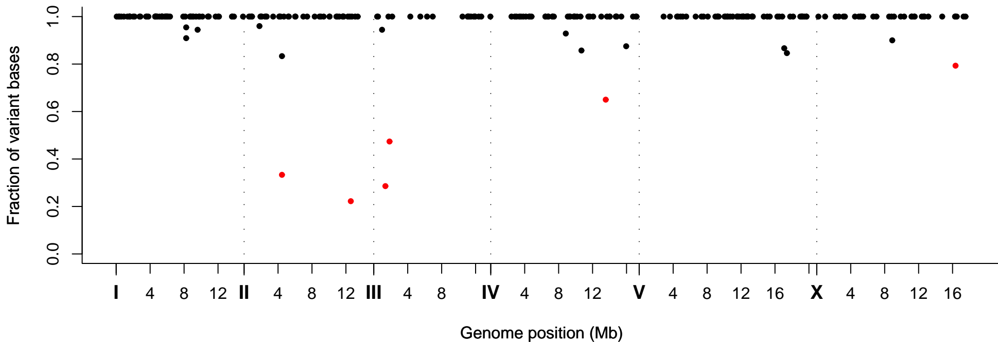
Fraction of Variant Bases at Position, Strain VC30185
