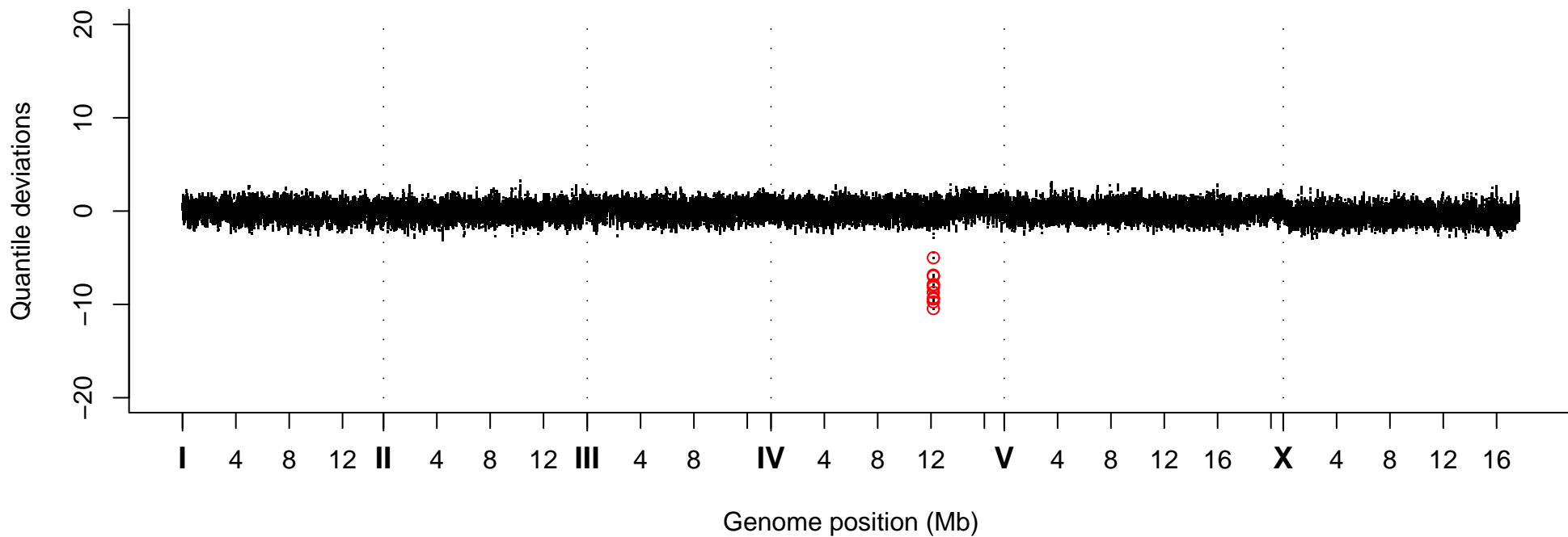
Quantile Deviations, Strain VC30185
