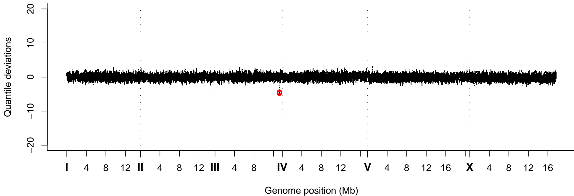
Quantile Deviations, Strain VC30201
