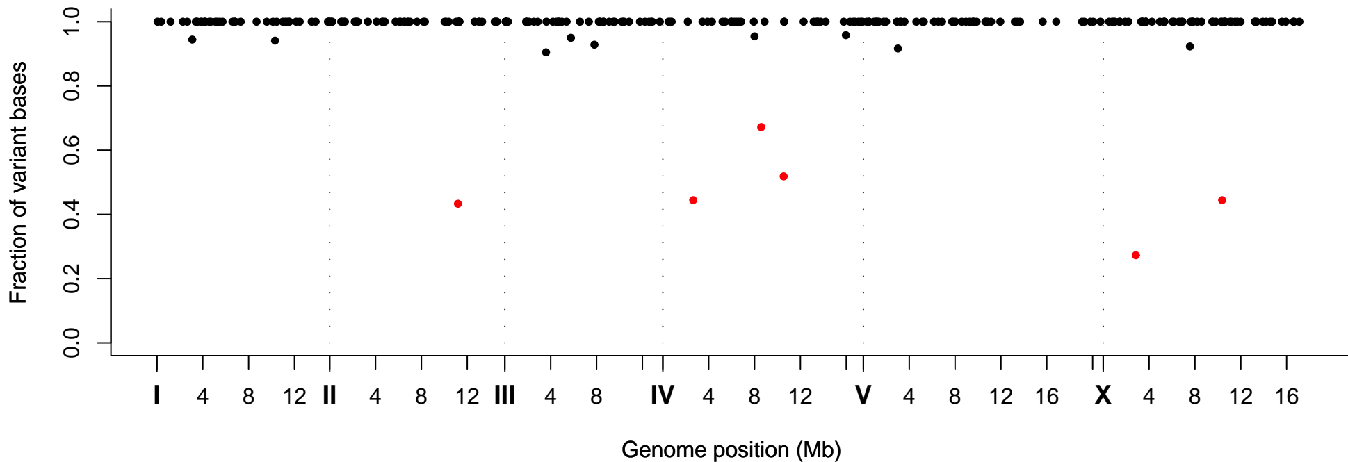
Fraction of Variant Bases at Position, Strain VC30201
