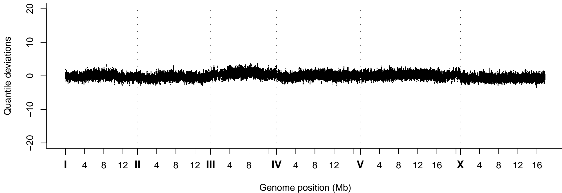
Quantile Deviations, Strain VC30210
