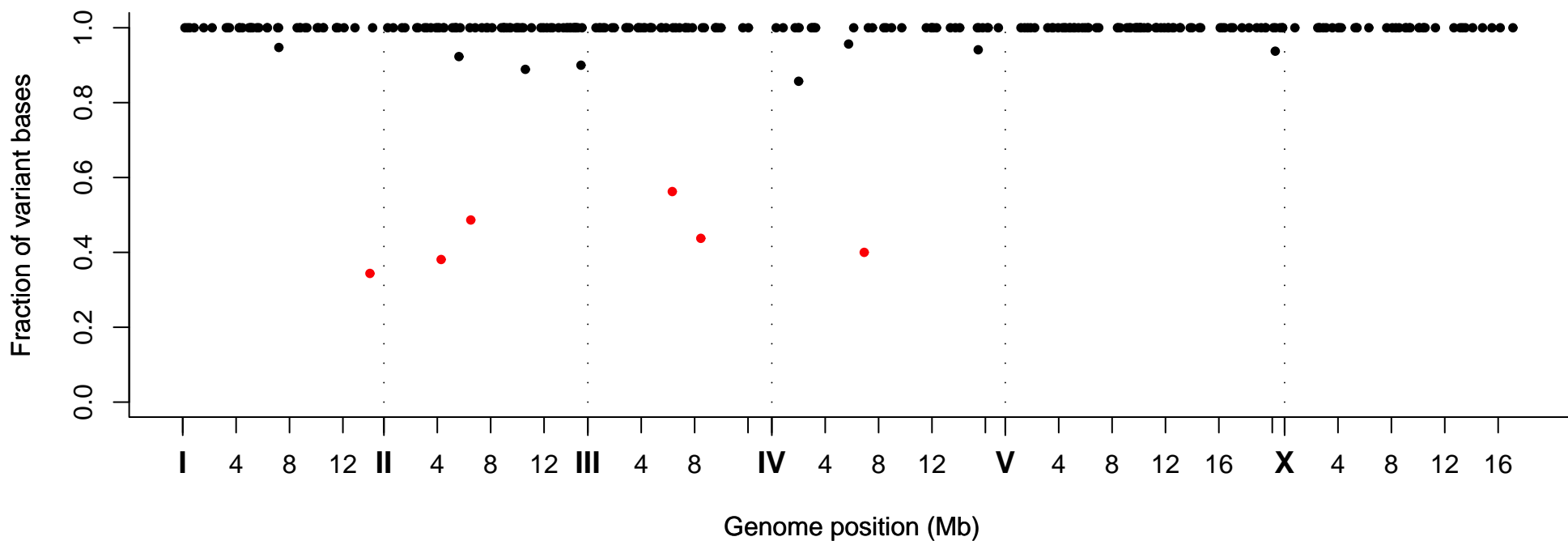
Fraction of Variant Bases at Position, Strain VC30210
