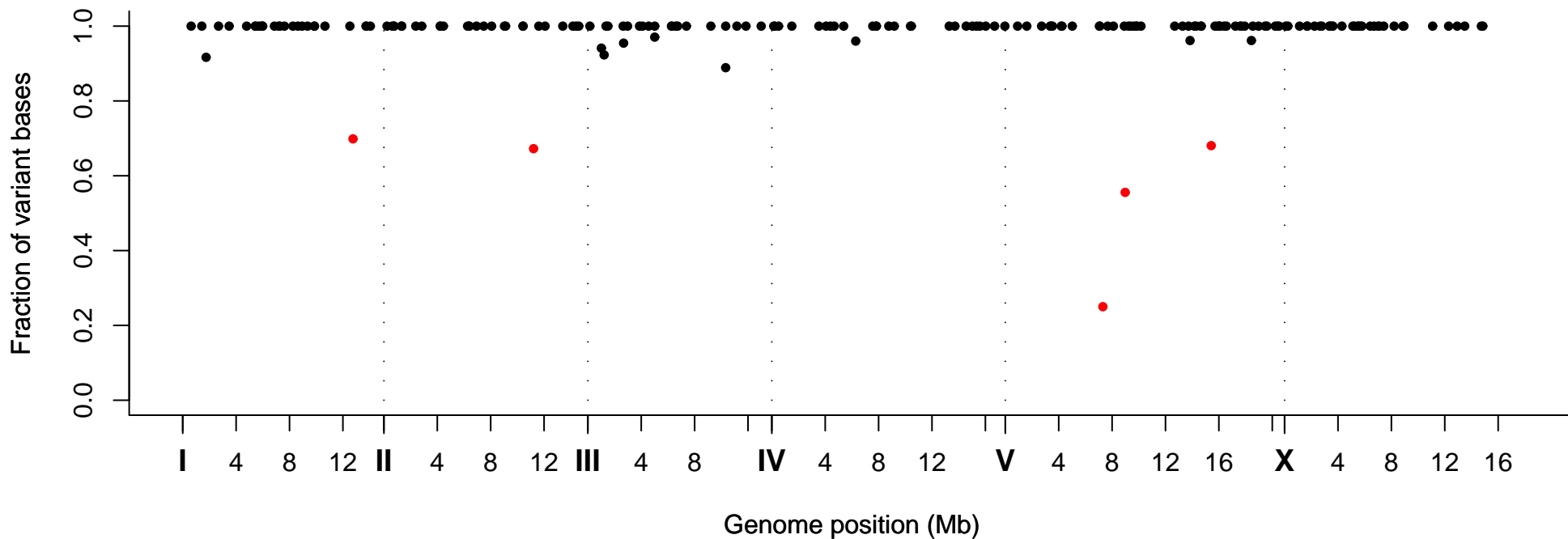
Fraction of Variant Bases at Position, Strain VC30216
