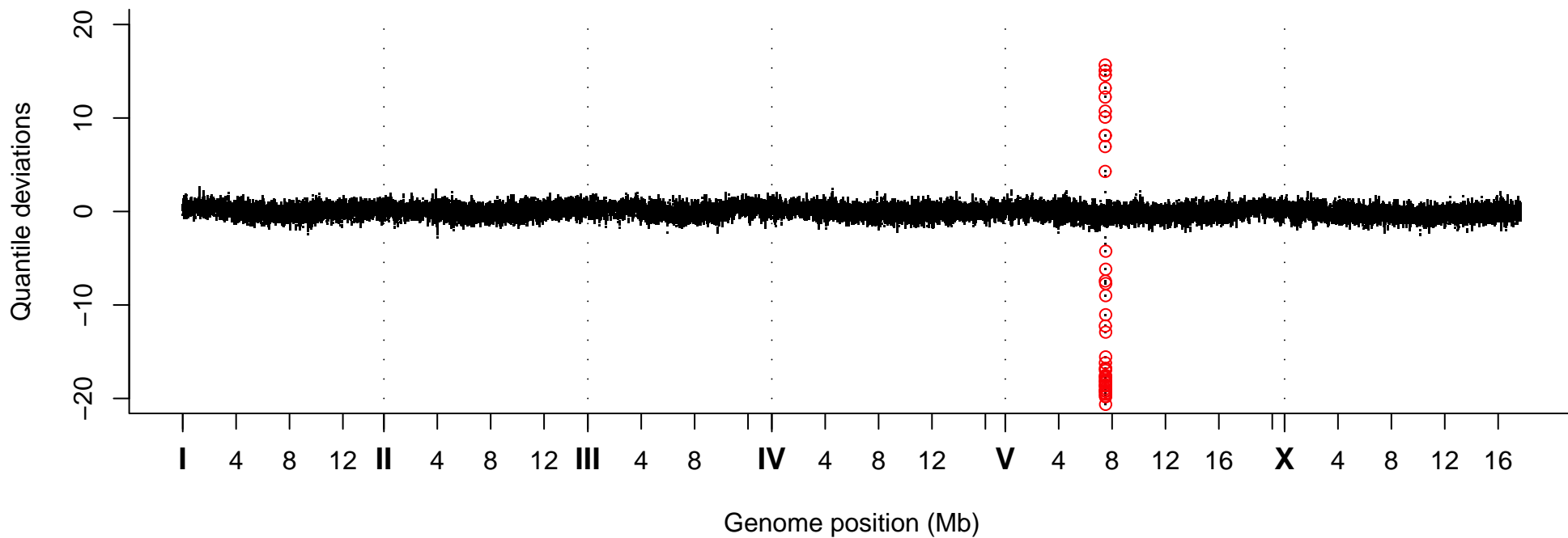
Quantile Deviations, Strain VC30216
