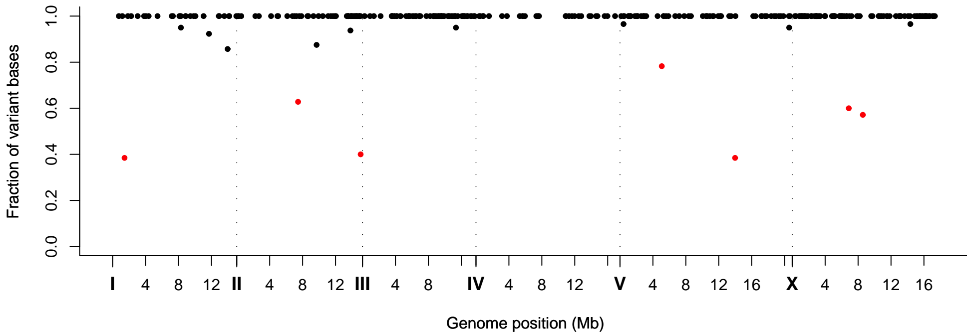
Fraction of Variant Bases at Position, Strain VC30217
