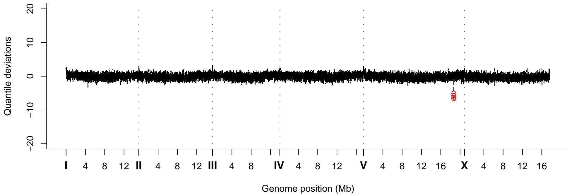
Quantile Deviations, Strain VC30217
