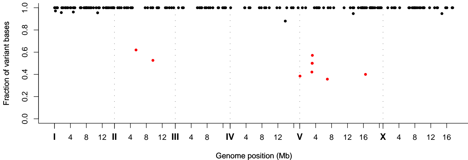
Fraction of Variant Bases at Position, Strain VC30219
