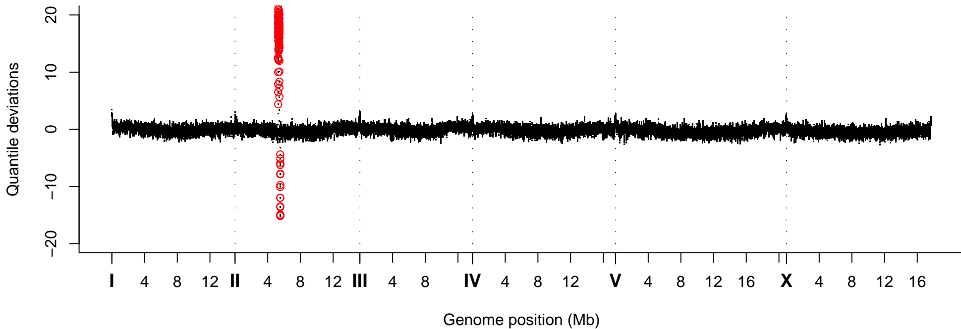
Quantile Deviations, Strain VC30219
