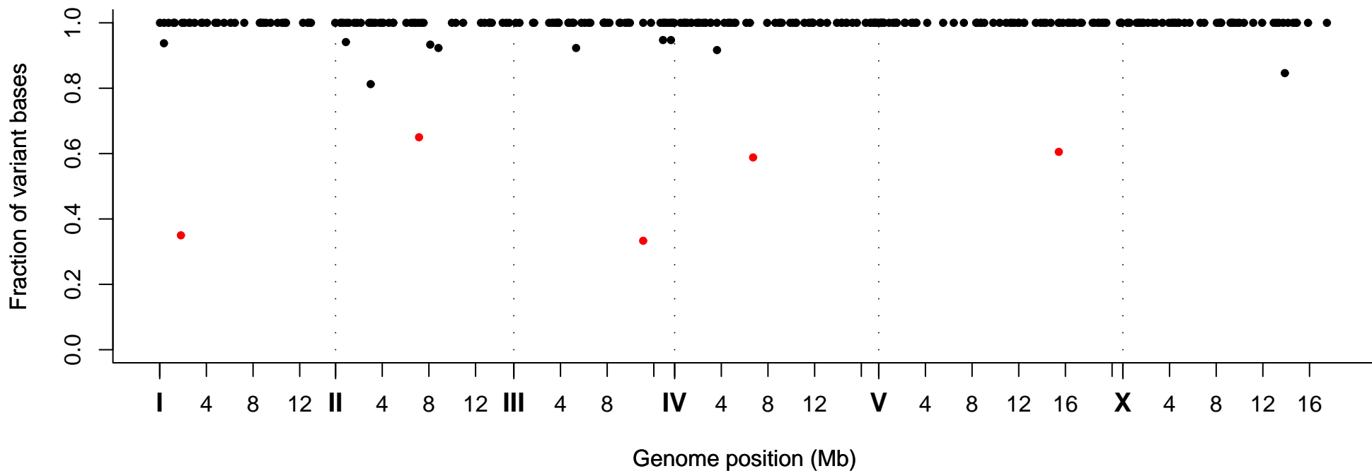
Fraction of Variant Bases at Position, Strain VC30221
