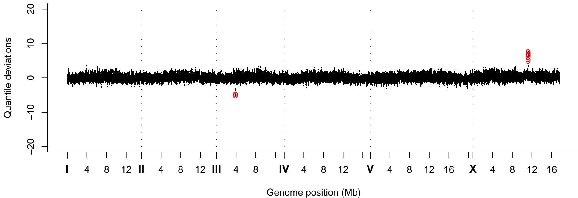
Quantile Deviations, Strain VC30221
