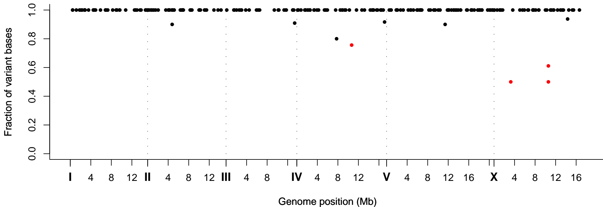
Fraction of Variant Bases at Position, Strain VC30224
