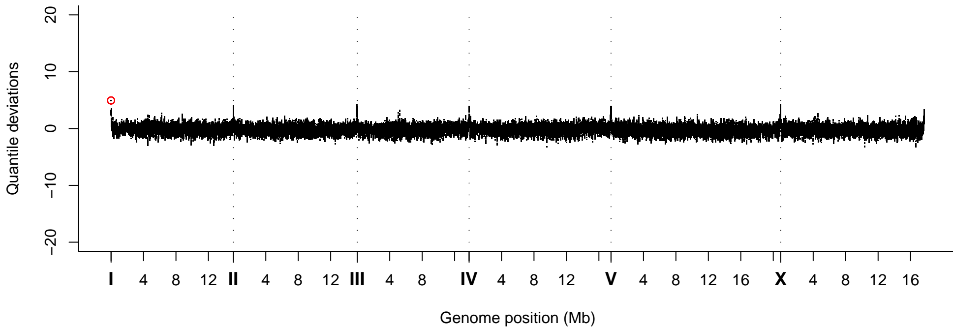
Quantile Deviations, Strain VC30224
