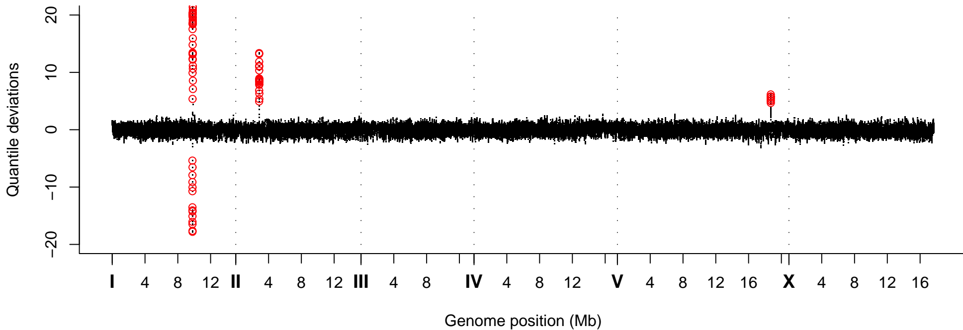
Quantile Deviations, Strain VC30237
