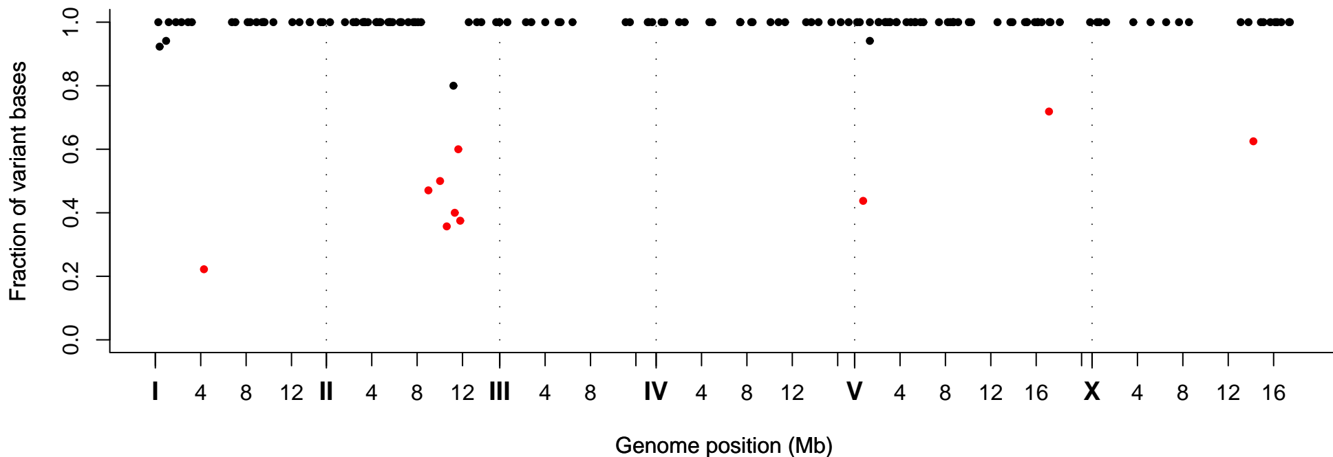
Fraction of Variant Bases at Position, Strain VC30237
