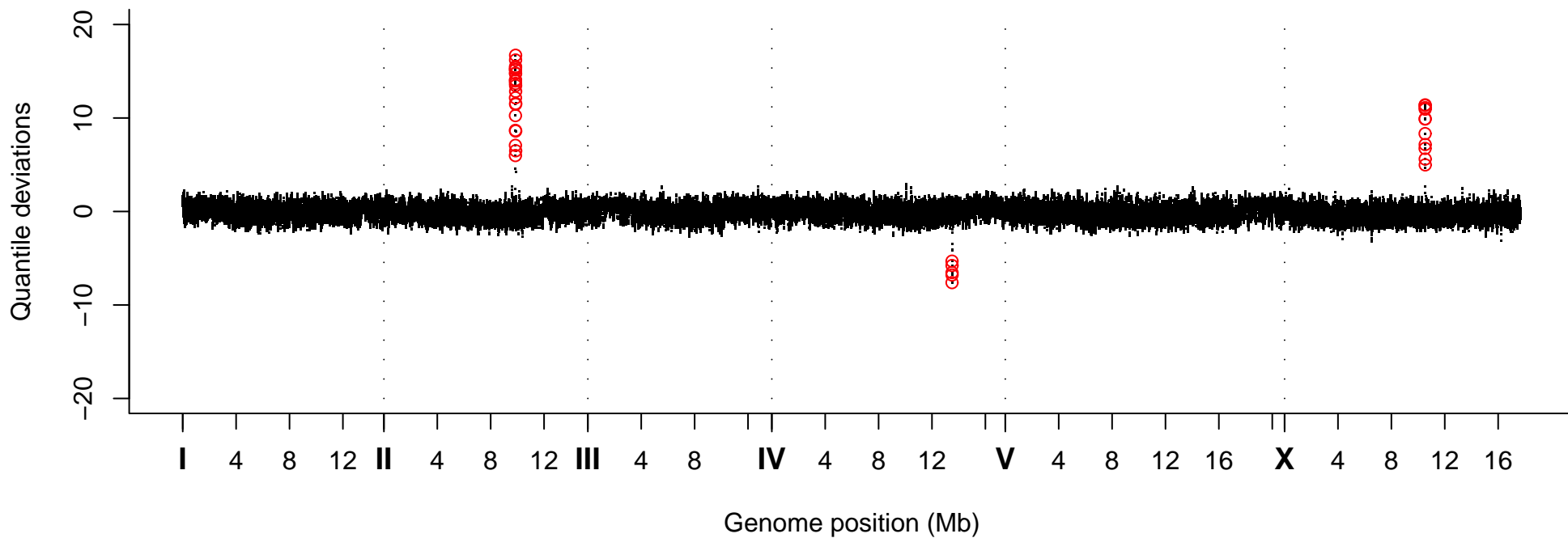
Quantile Deviations, Strain VC30240
