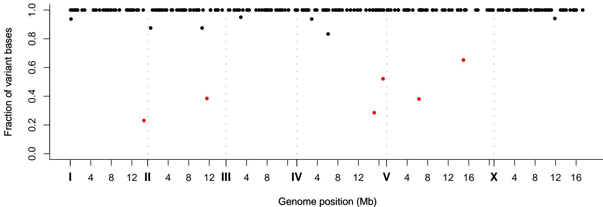
Fraction of Variant Bases at Position, Strain VC30240
