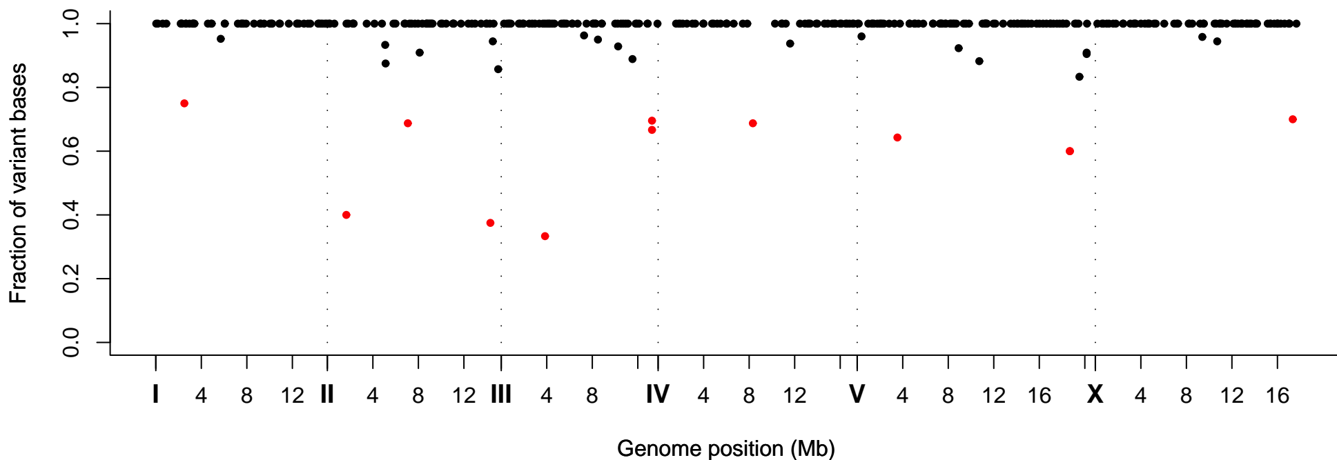
Fraction of Variant Bases at Position, Strain VC30245
