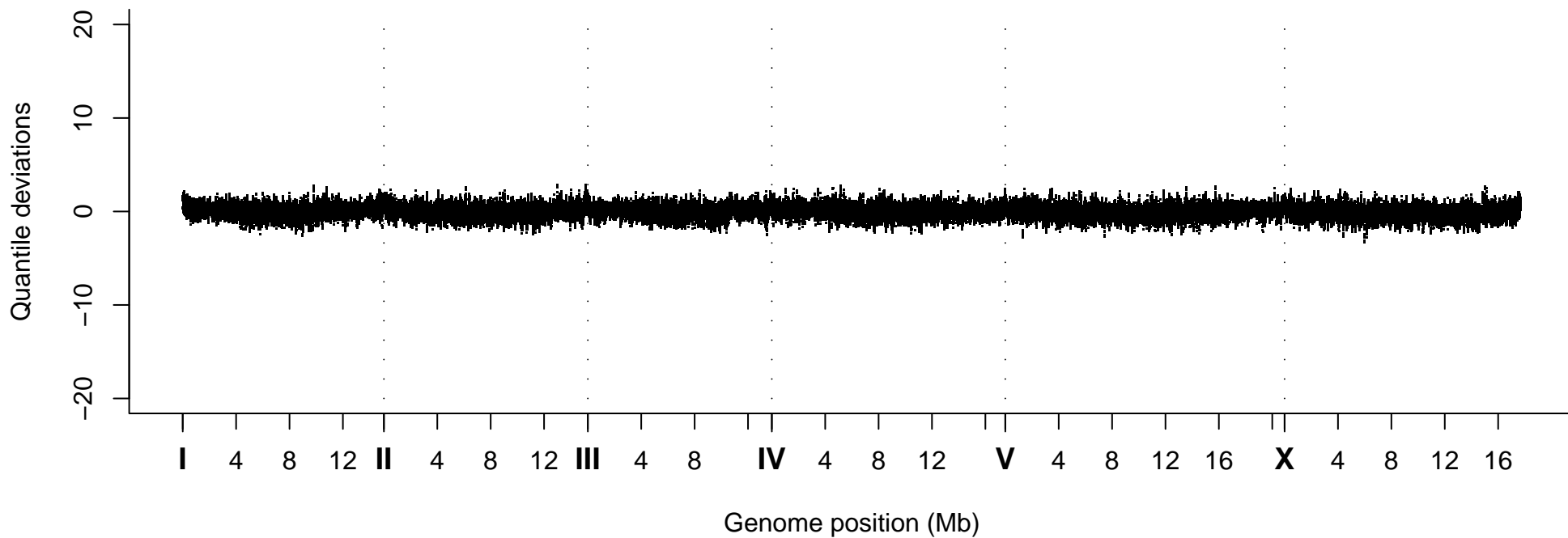
Quantile Deviations, Strain VC30245
