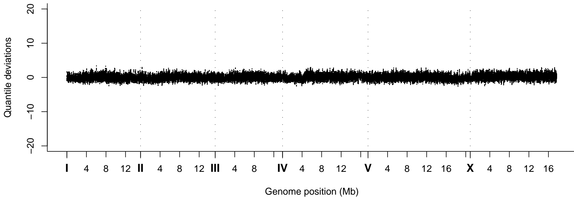
Quantile Deviations, Strain VC30247
