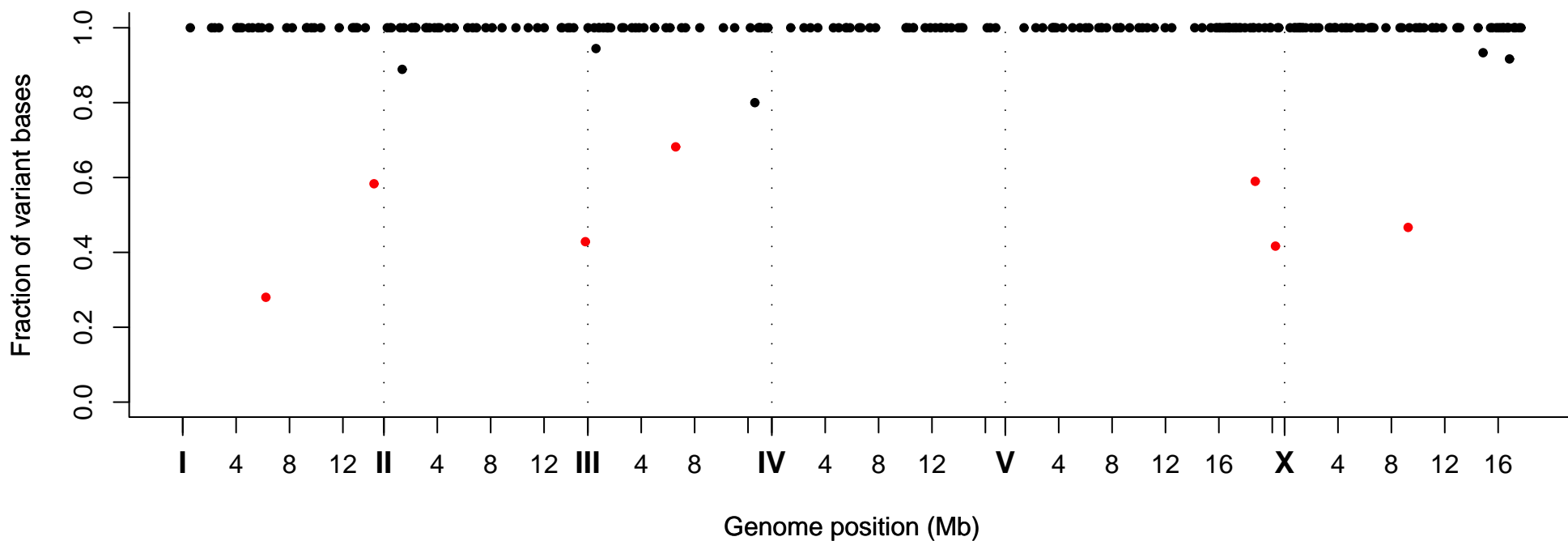
Fraction of Variant Bases at Position, Strain VC30247
