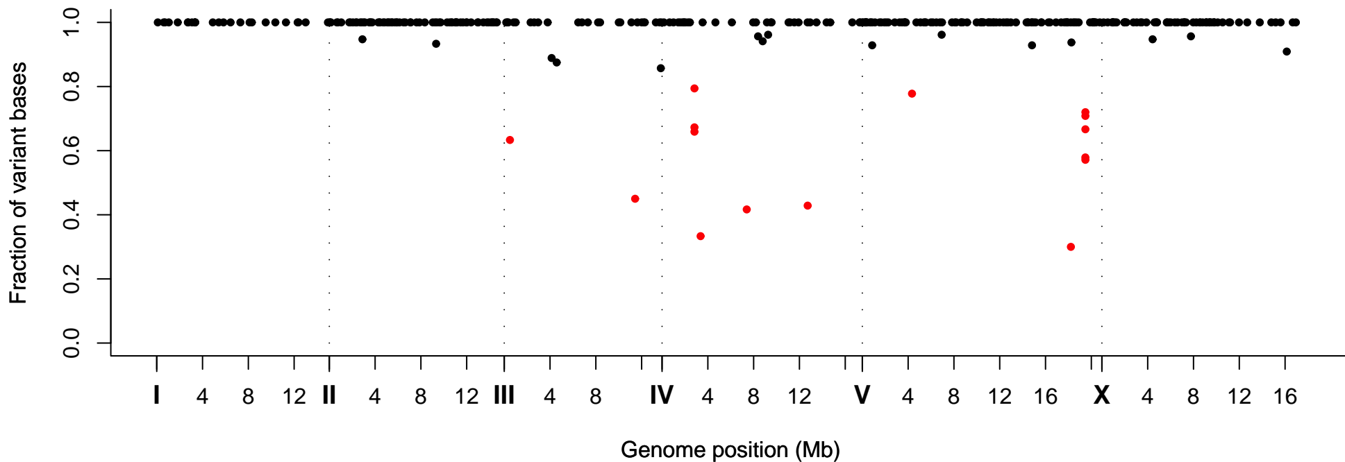
Fraction of Variant Bases at Position, Strain VC30250
