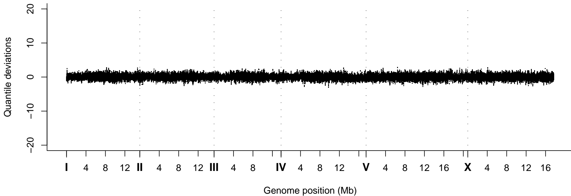
Quantile Deviations, Strain VC30250
