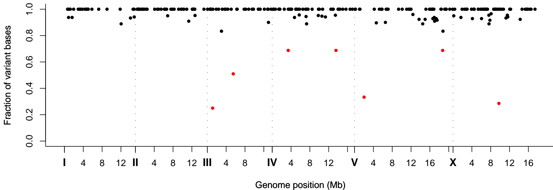
Fraction of Variant Bases at Position, Strain VC30251
