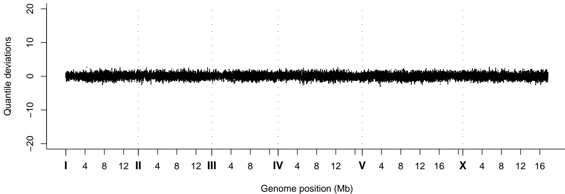
Quantile Deviations, Strain VC30251
