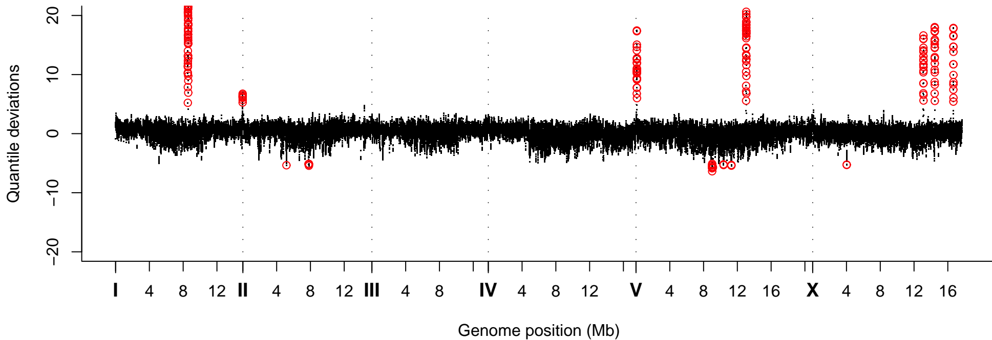
Quantile Deviations, Strain VC30256
