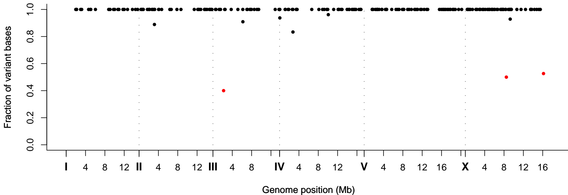
Fraction of Variant Bases at Position, Strain VC30256
