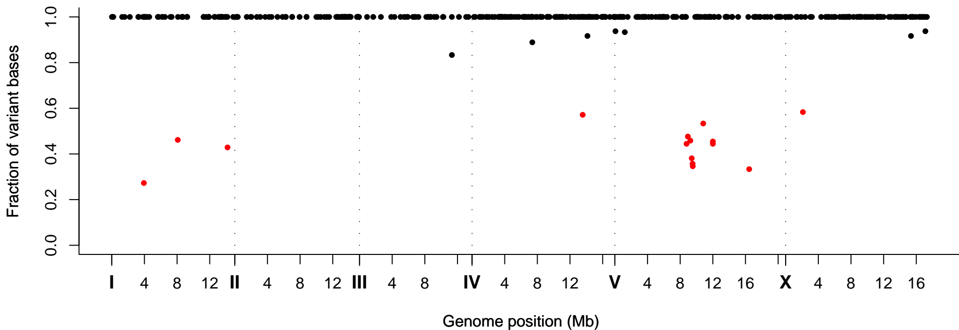
Fraction of Variant Bases at Position, Strain VC30259
