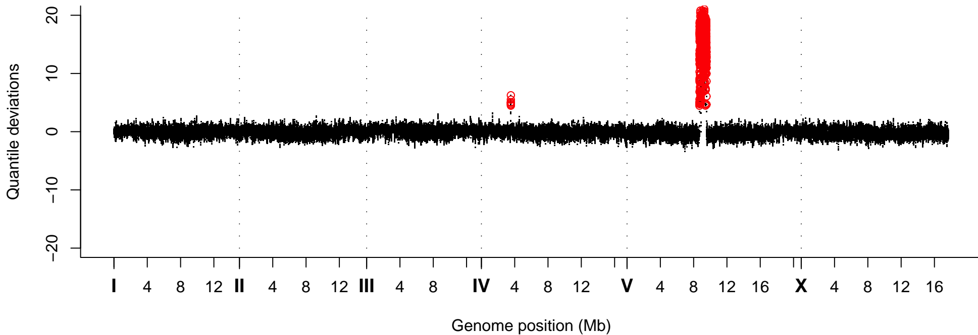
Quantile Deviations, Strain VC30259
