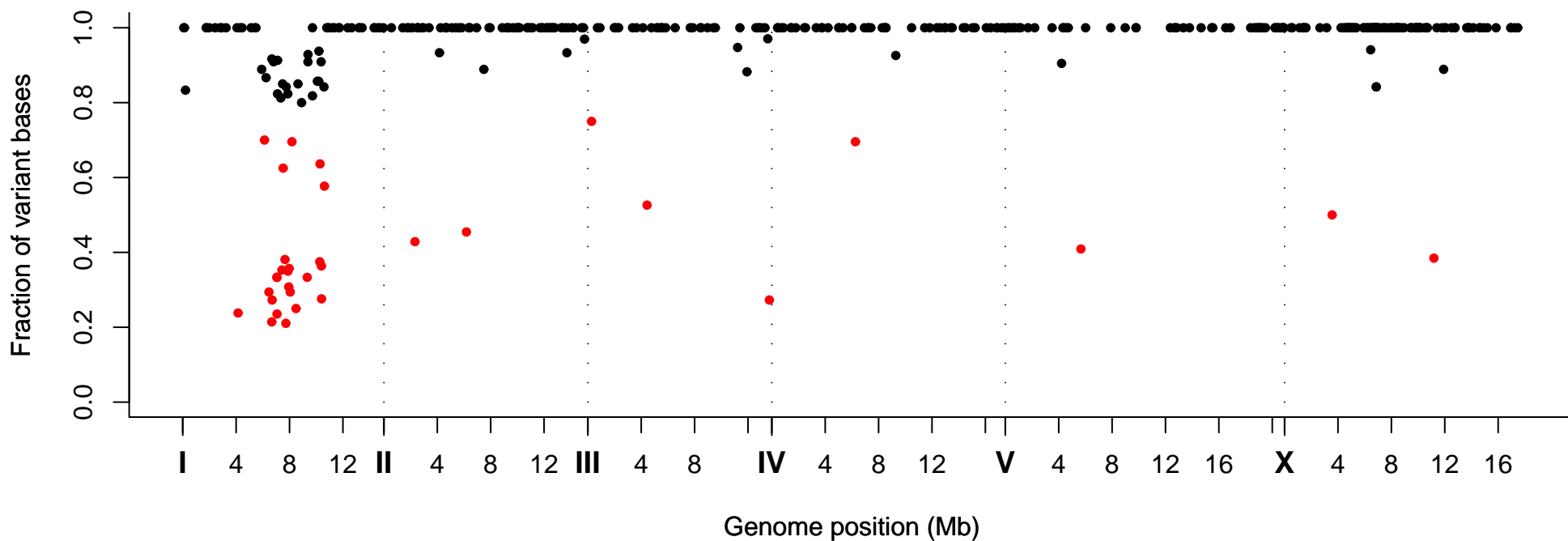
Fraction of Variant Bases at Position, Strain VC40000
