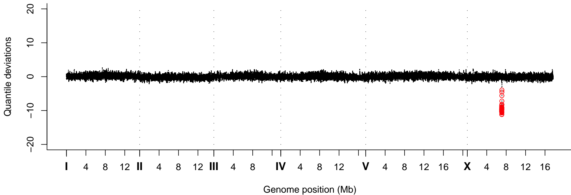
Quantile Deviations, Strain VC40001
