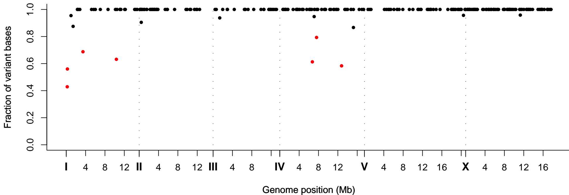
Fraction of Variant Bases at Position, Strain VC40001
