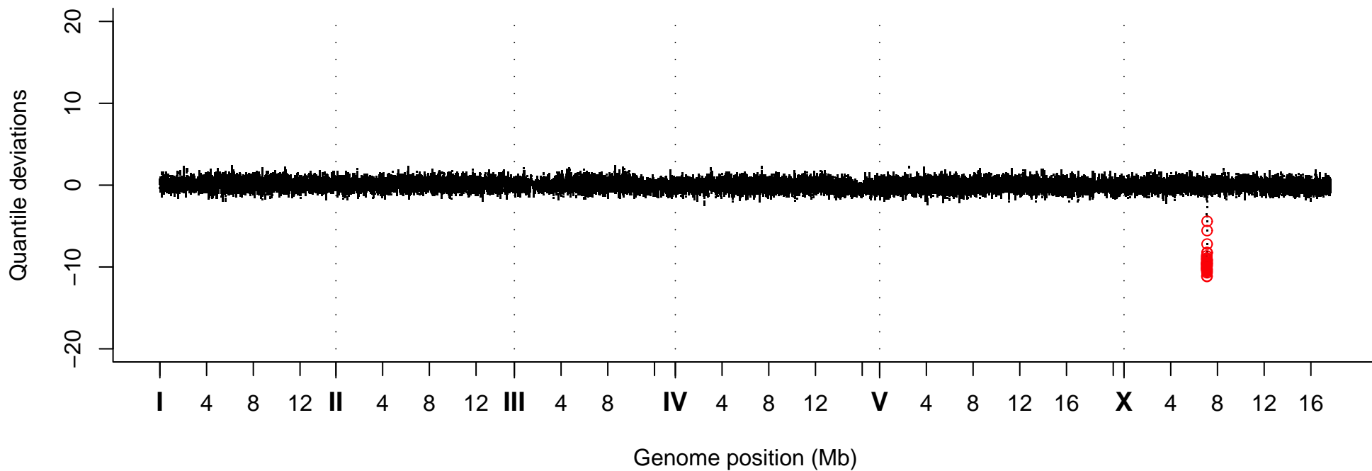
Quantile Deviations, Strain VC40003
