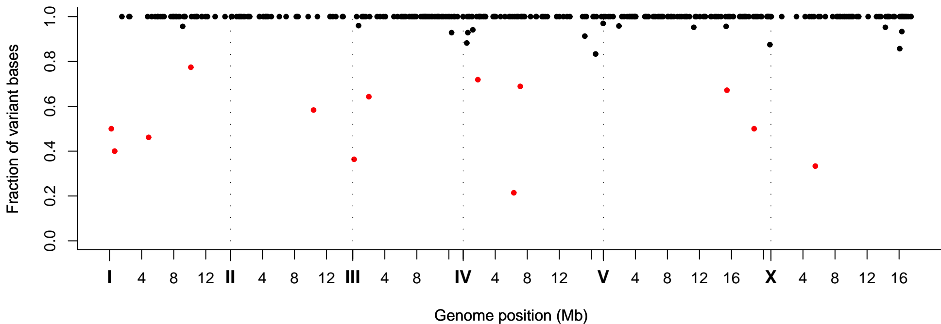
Fraction of Variant Bases at Position, Strain VC40003
