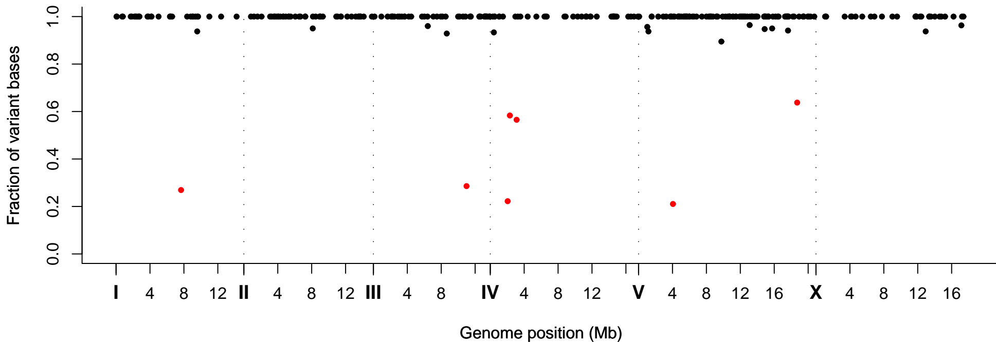
Fraction of Variant Bases at Position, Strain VC40012
