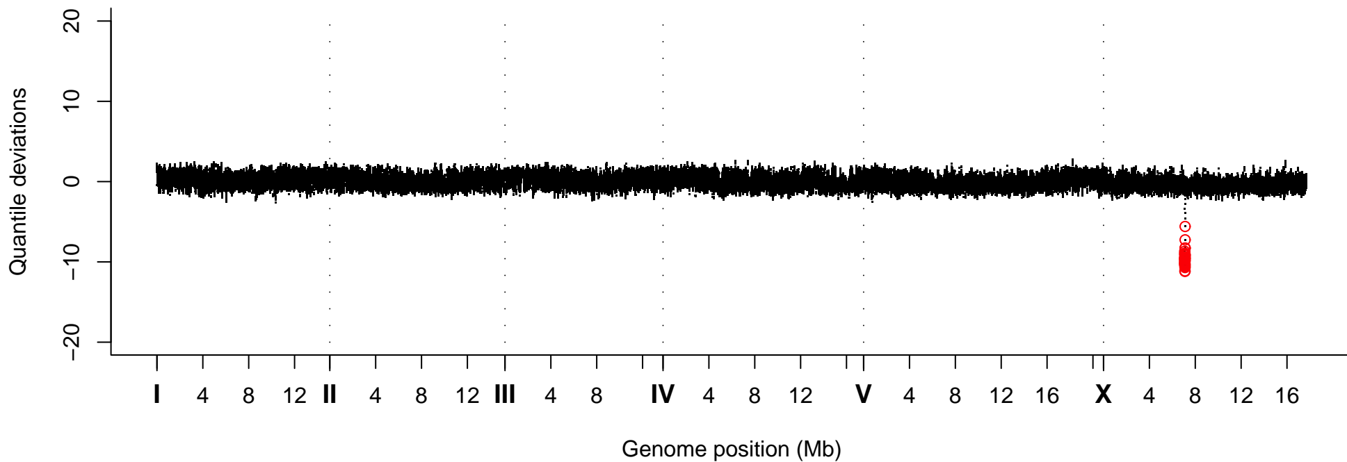
Quantile Deviations, Strain VC40012
