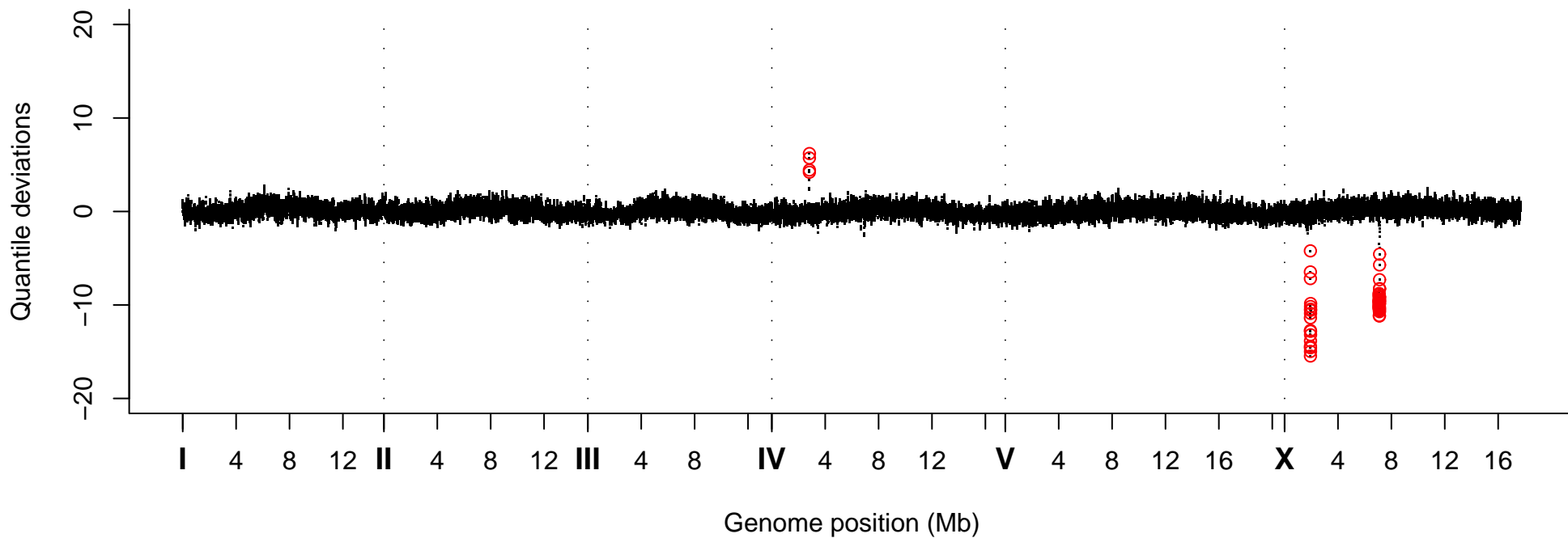
Quantile Deviations, Strain VC40017
