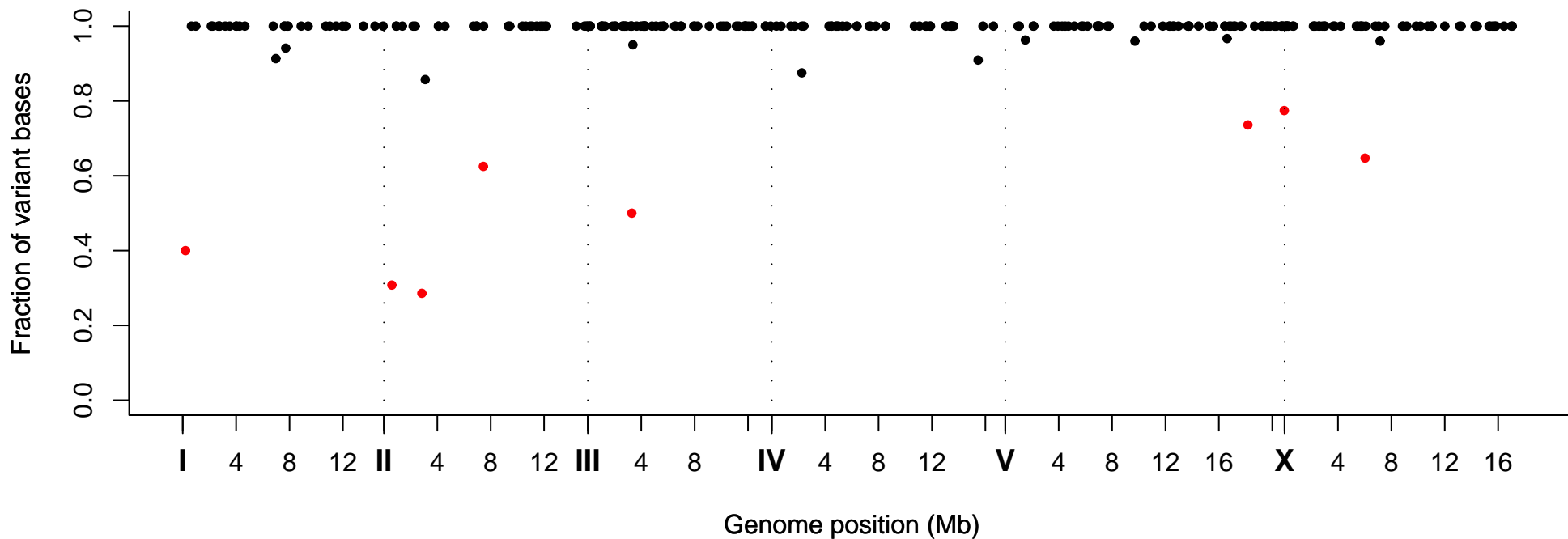
Fraction of Variant Bases at Position, Strain VC40017
