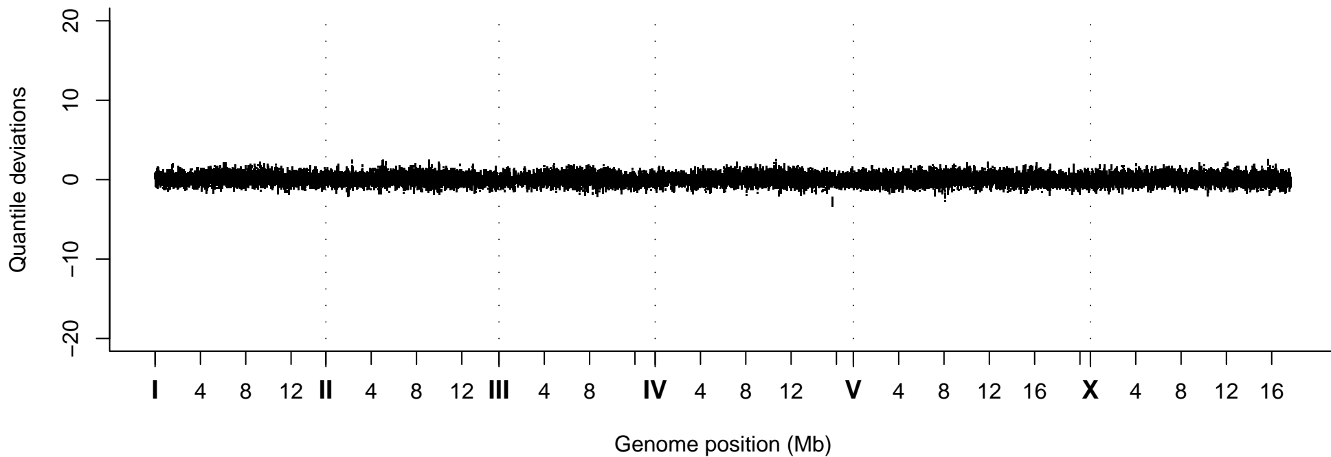
Quantile Deviations, Strain VC40019
