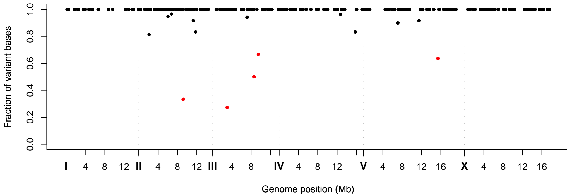
Fraction of Variant Bases at Position, Strain VC40019
