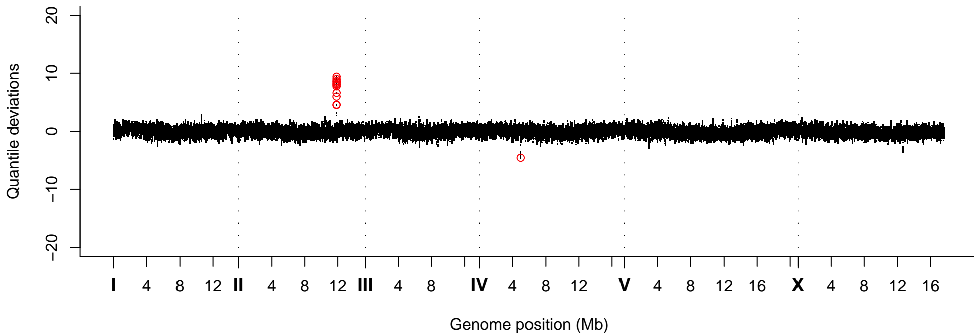
Quantile Deviations, Strain VC40024
