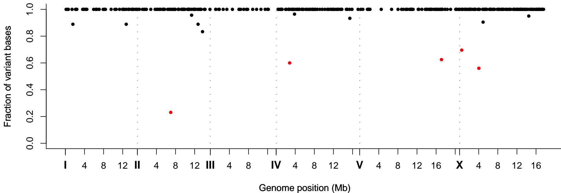
Fraction of Variant Bases at Position, Strain VC40024
