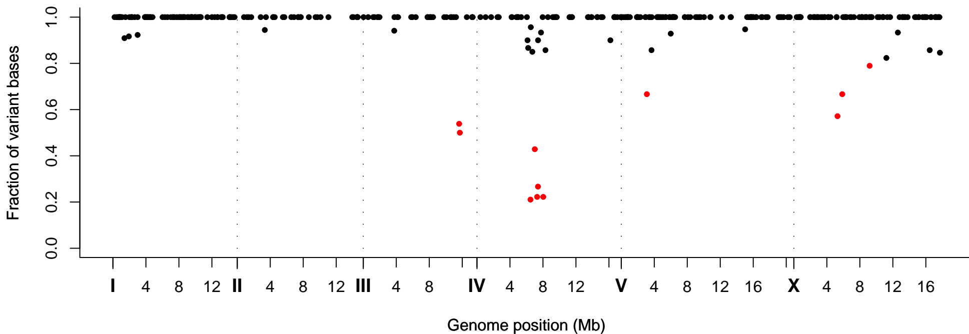
Fraction of Variant Bases at Position, Strain VC40038
