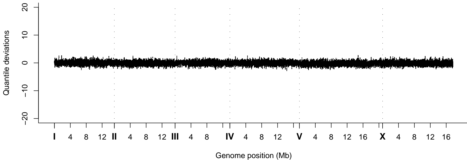
Quantile Deviations, Strain VC40038
