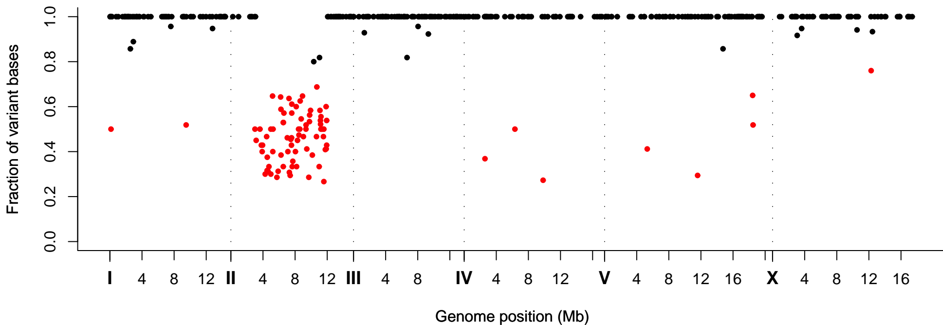
Fraction of Variant Bases at Position, Strain VC40040
