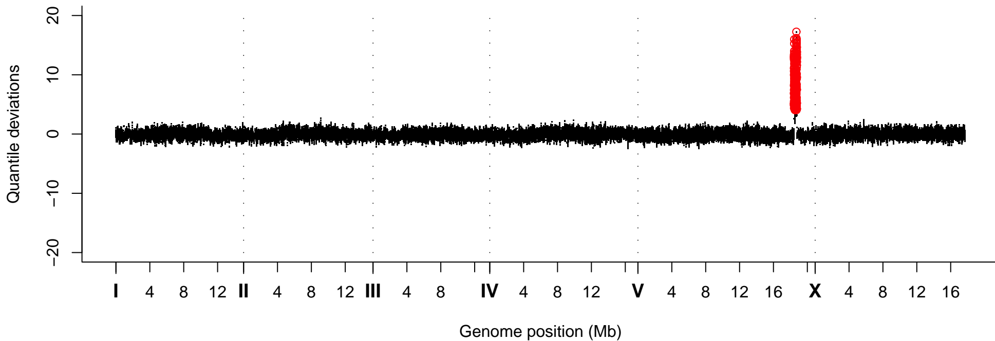
Quantile Deviations, Strain VC40040
