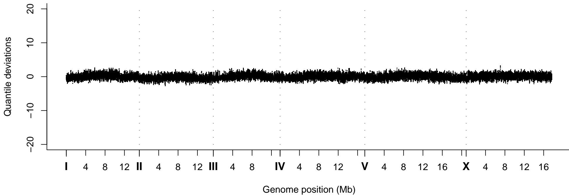
Quantile Deviations, Strain VC40041
