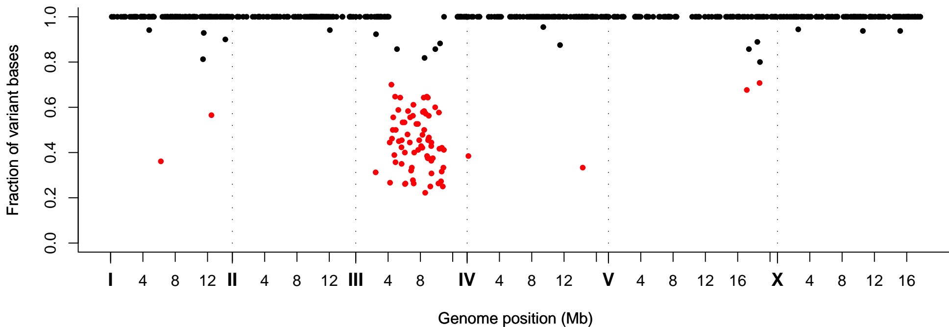
Fraction of Variant Bases at Position, Strain VC40041
