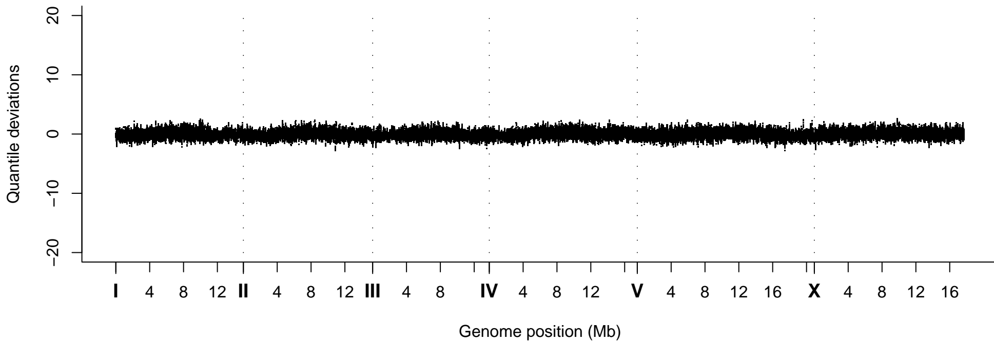
Quantile Deviations, Strain VC40042
