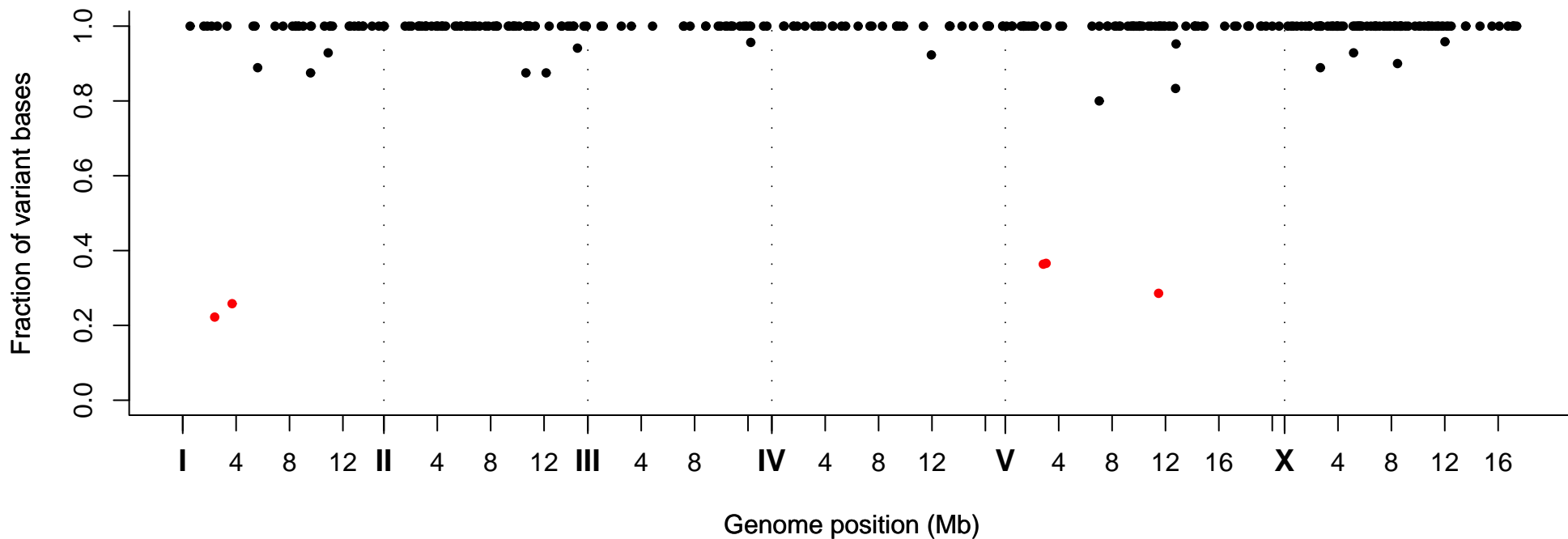
Fraction of Variant Bases at Position, Strain VC40042
