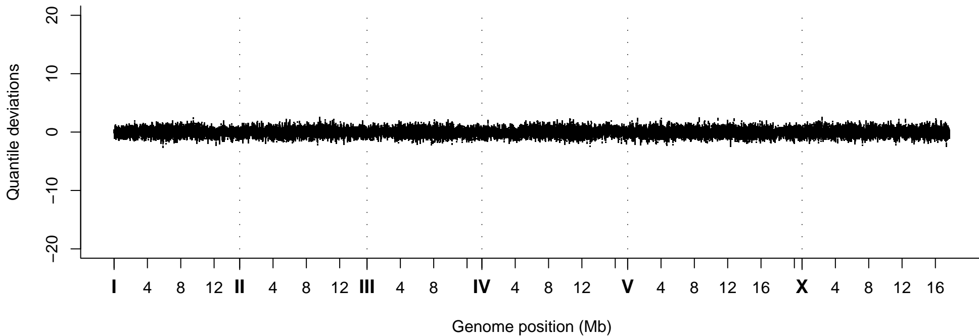
Quantile Deviations, Strain VC40047
