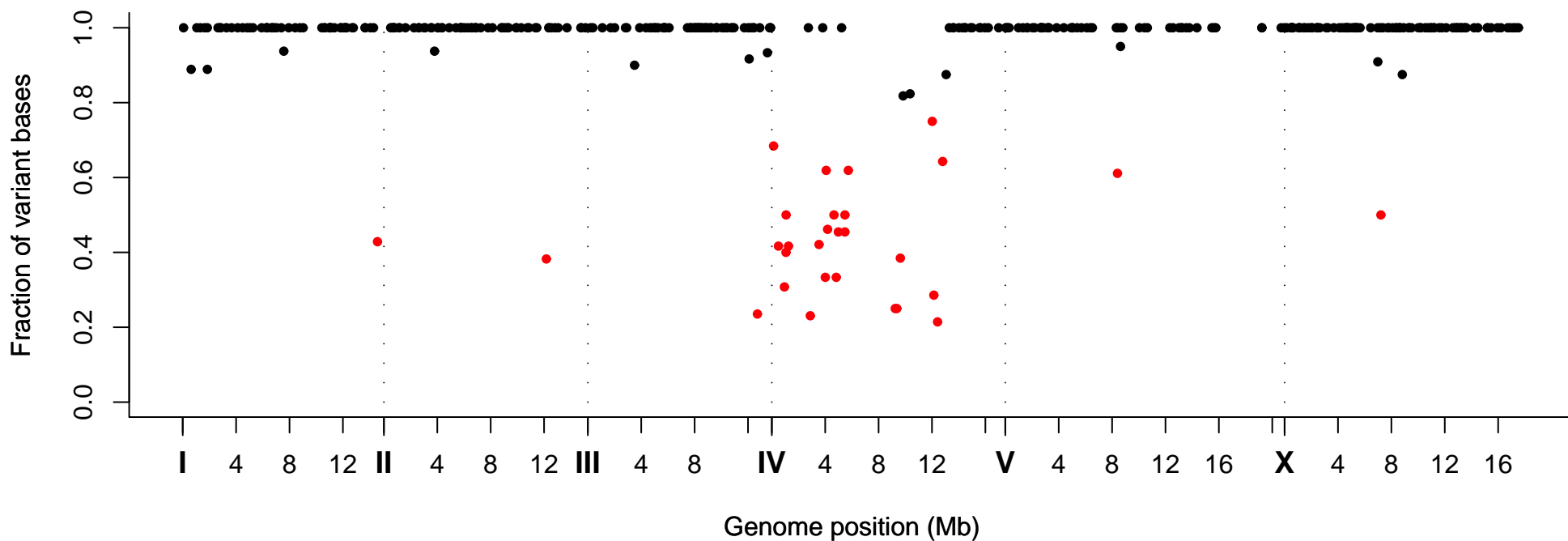
Fraction of Variant Bases at Position, Strain VC40047
