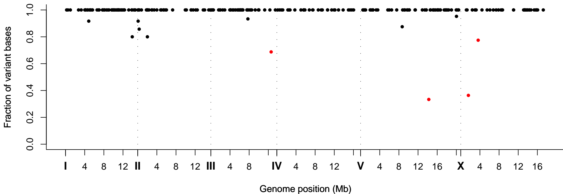
Fraction of Variant Bases at Position, Strain VC40052
