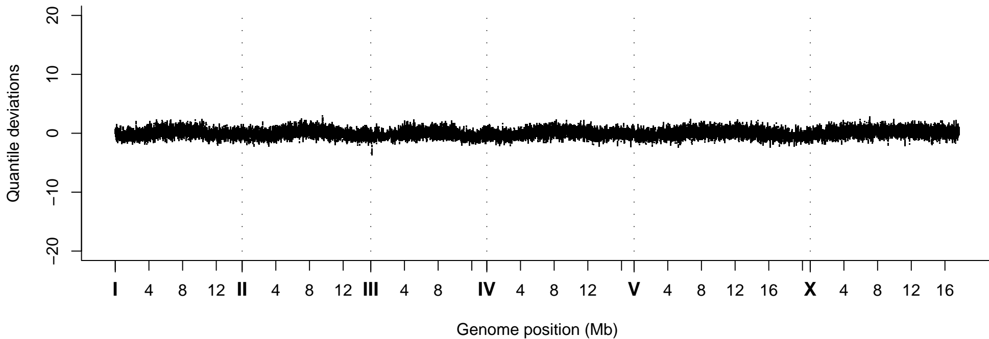
Quantile Deviations, Strain VC40054
