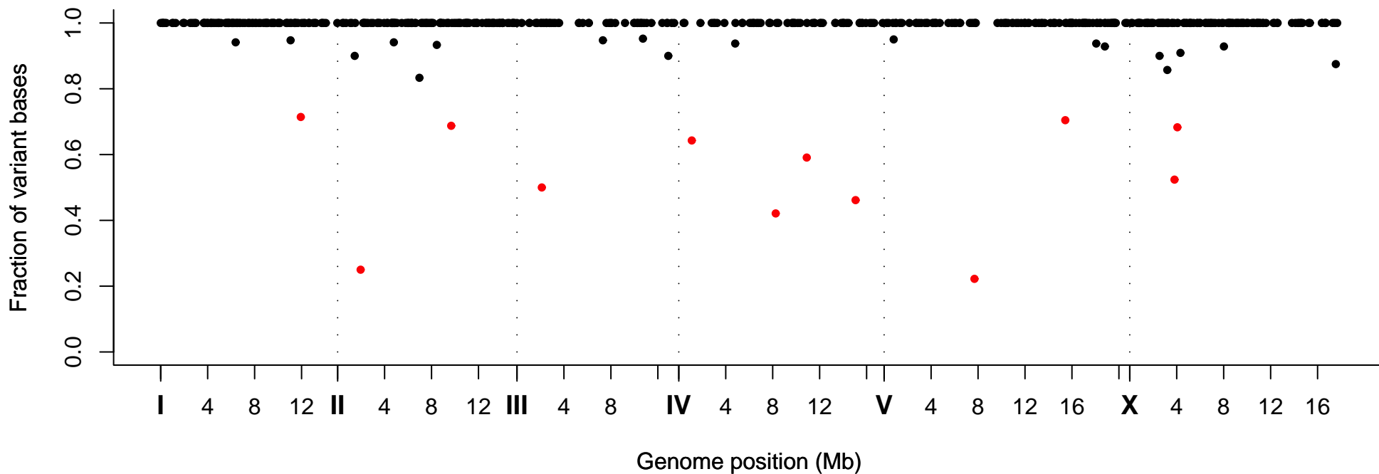
Fraction of Variant Bases at Position, Strain VC40054
