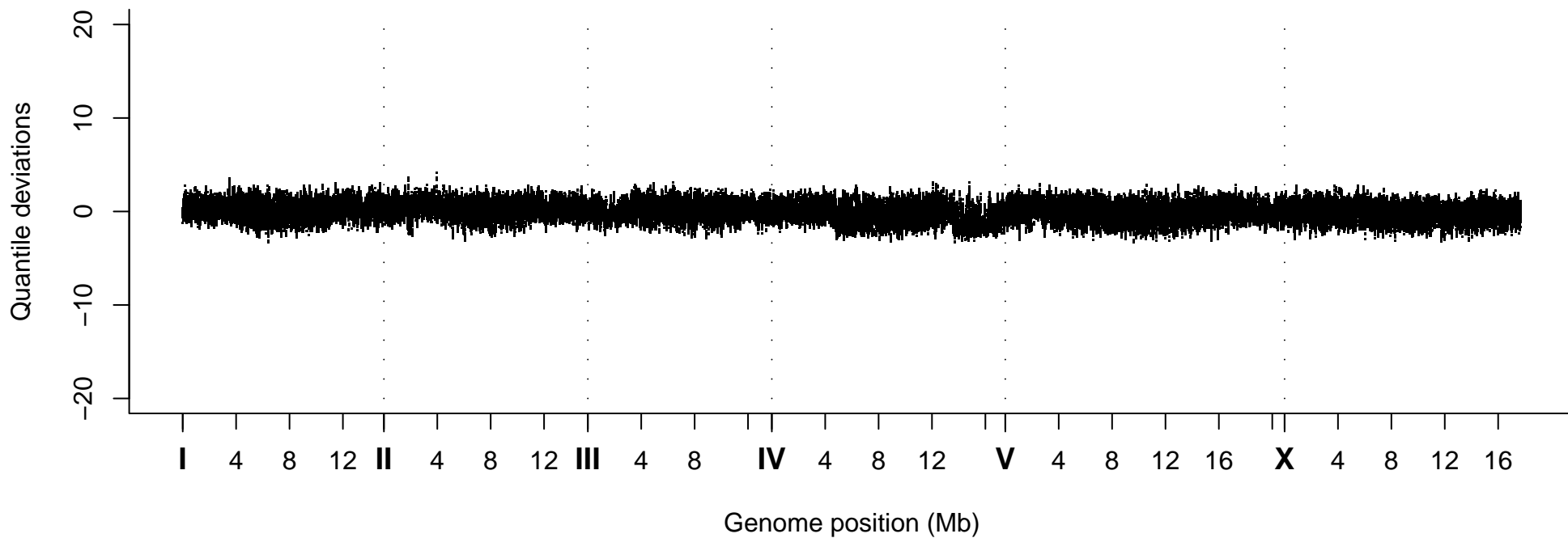
Quantile Deviations, Strain VC40061
