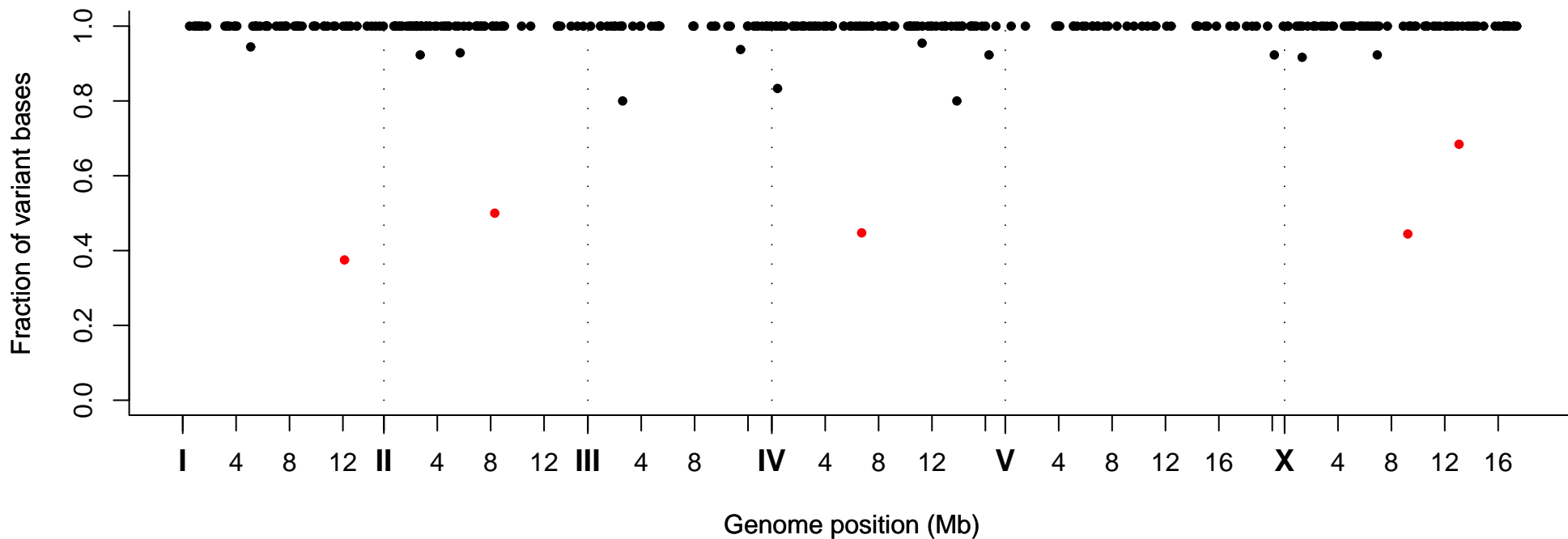
Fraction of Variant Bases at Position, Strain VC40064
