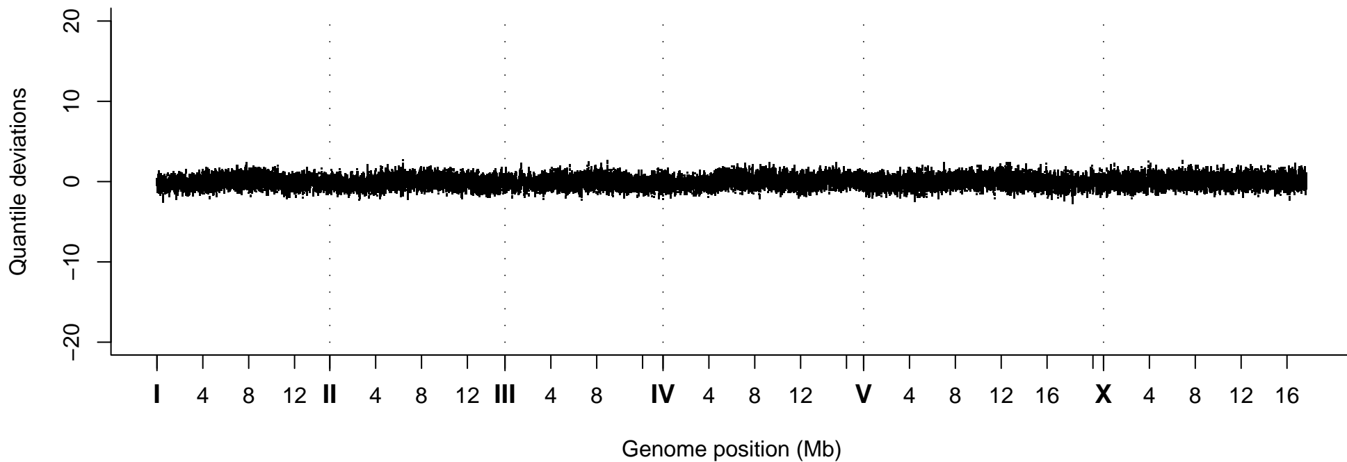
Quantile Deviations, Strain VC40064
