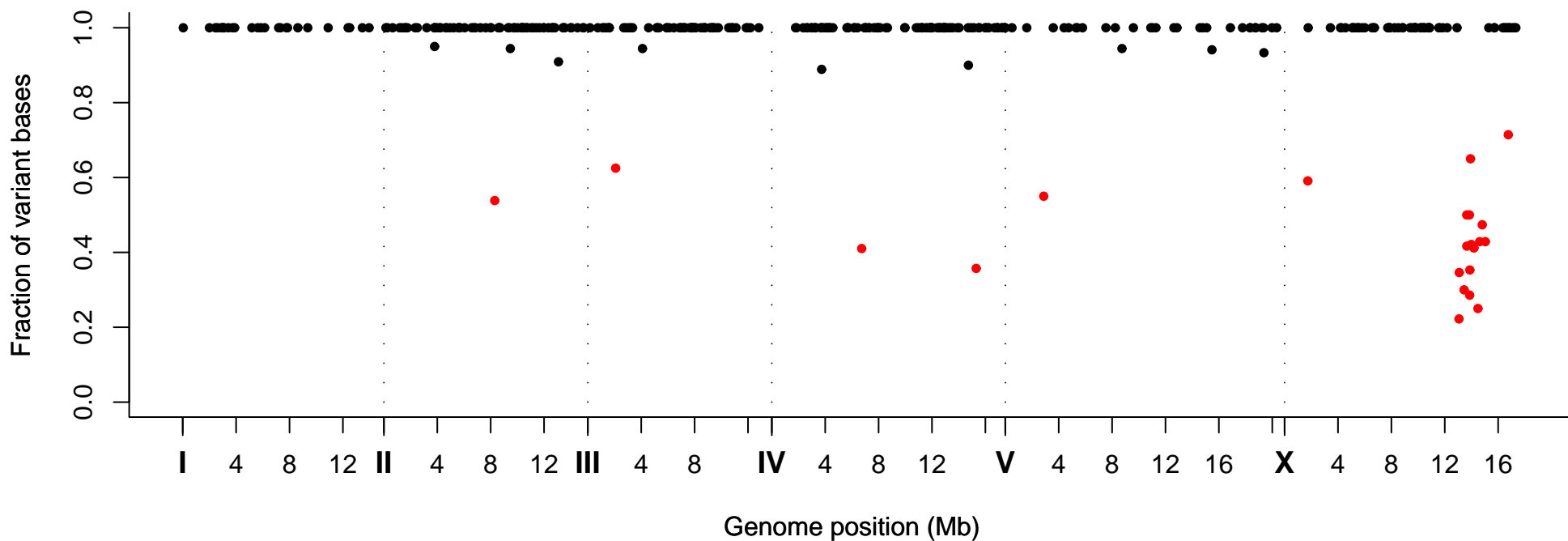
Fraction of Variant Bases at Position, Strain VC40074
