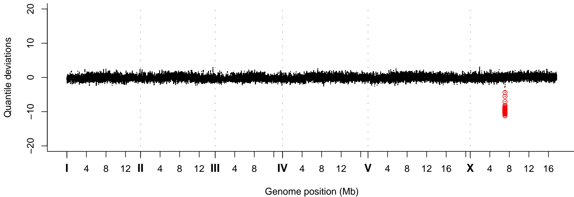
Quantile Deviations, Strain VC40074
