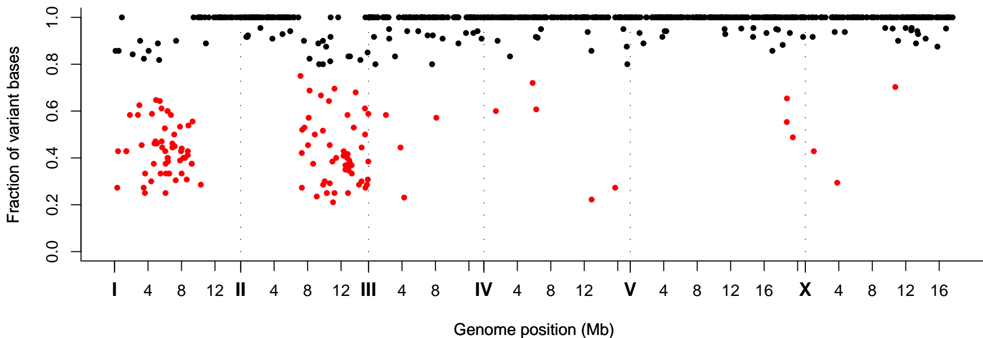
Fraction of Variant Bases at Position, Strain VC40076
