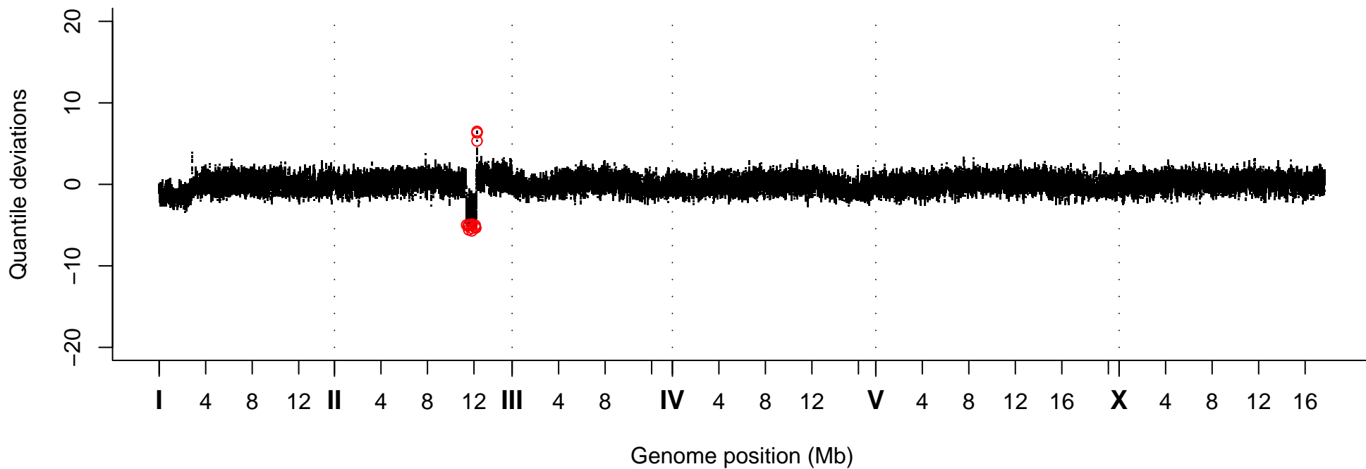
Quantile Deviations, Strain VC40076
